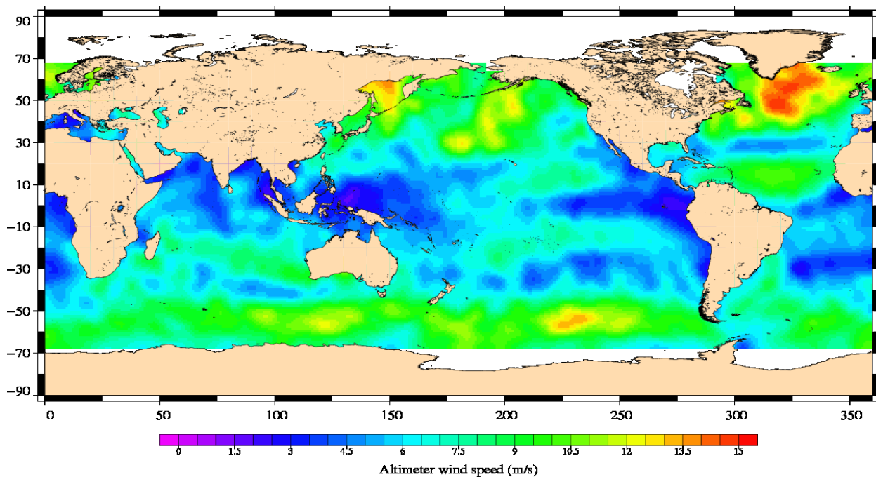
Jason-1 Cycle 335 04/02/2011 - 14/02/2011
