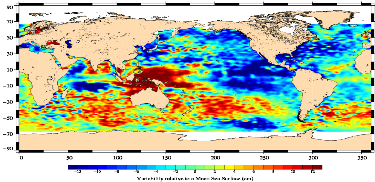
Jason-1 Cycle 335 04/02/2011 – 14/02/2011
