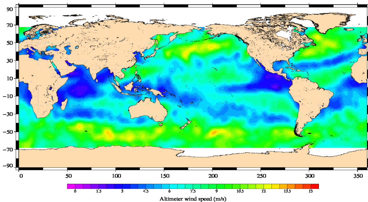
Jason-1 Cycle 340 25/03/2011 – 04/04/2011
