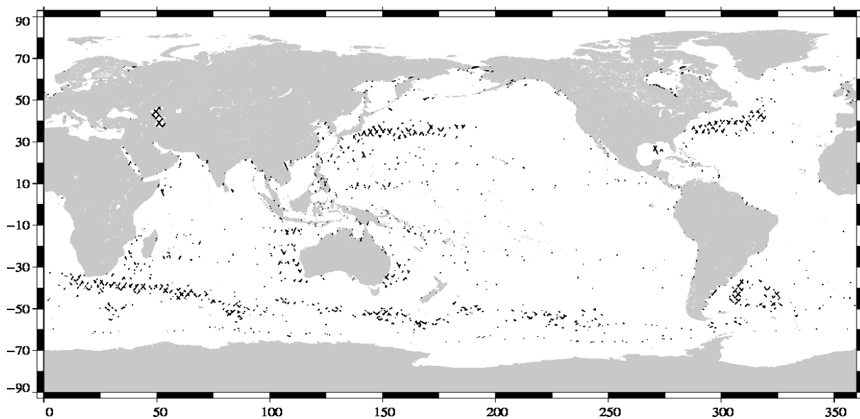
Valid data: (SSH – MSS) differences greater than 30 cm Jason-1 Cycle 351 (12/07/2011 / 22/07/2011)
