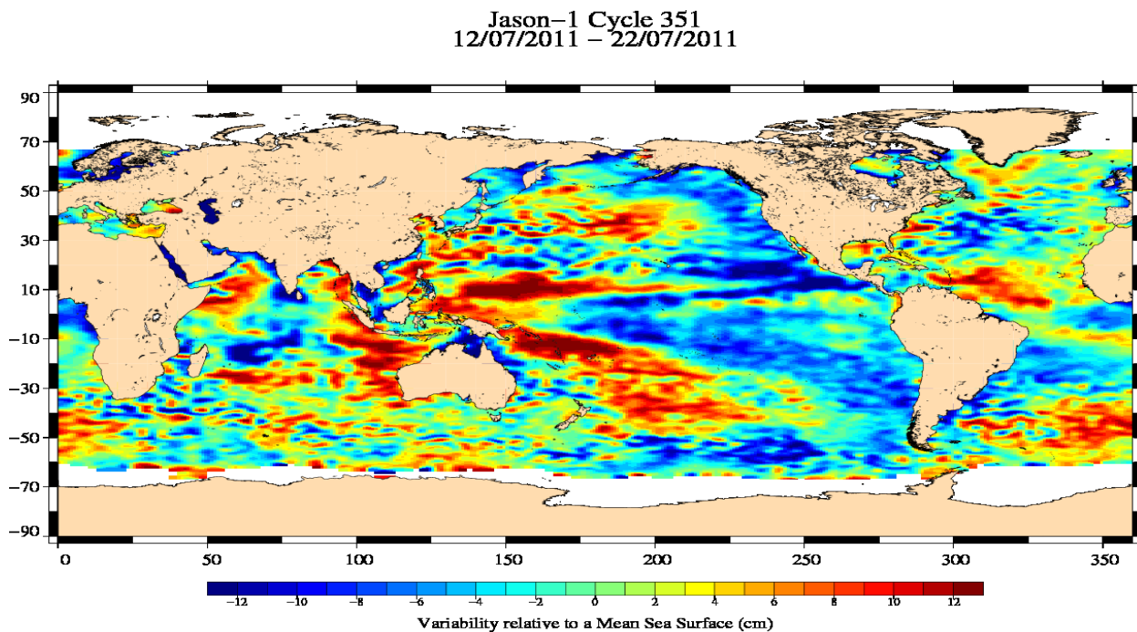
Valid data: (SSH – MSS) differences greater than 30 cm Jason-1 Cycle 351 (12/07/2011 / 22/07/2011)
