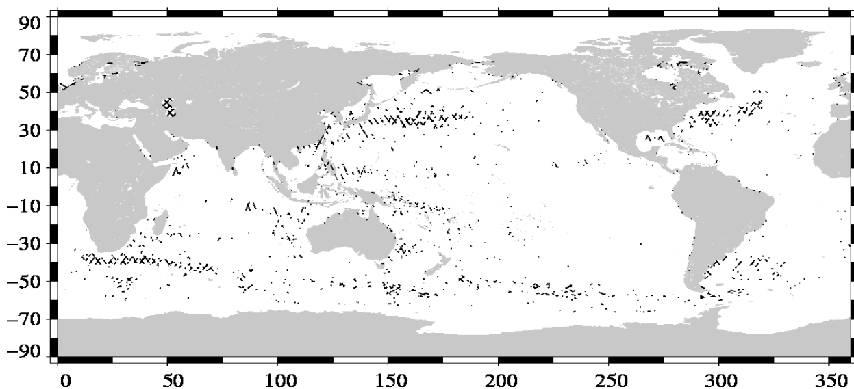
Valid data: (SSH – MSS) differences greater than 30 cm Jason-1 Cycle 359 (30/09/2011 / 09/10/2011)
