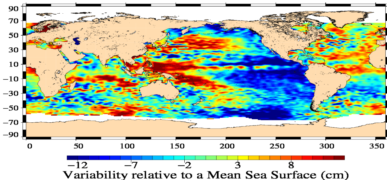
Jason-1 Cycle 361 19/10/2011 – 29/10/2011
