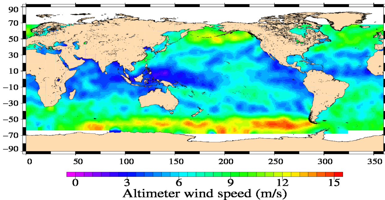
Jason-1 Cycle 361 19/10/2011 – 29/10/2011
