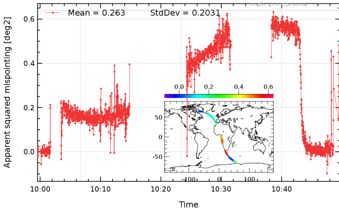
Jason-1 GDR Cycle 363 pass 198 (ocean data)
