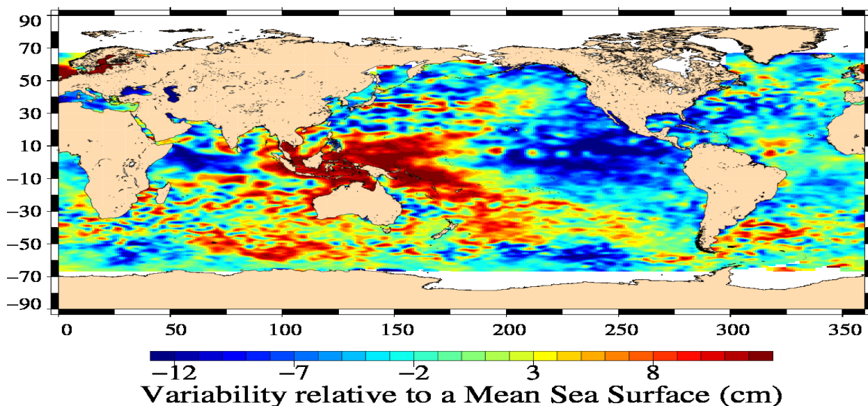
Jason-1 Cycle 369 07/01/2012 – 17/01/2012
