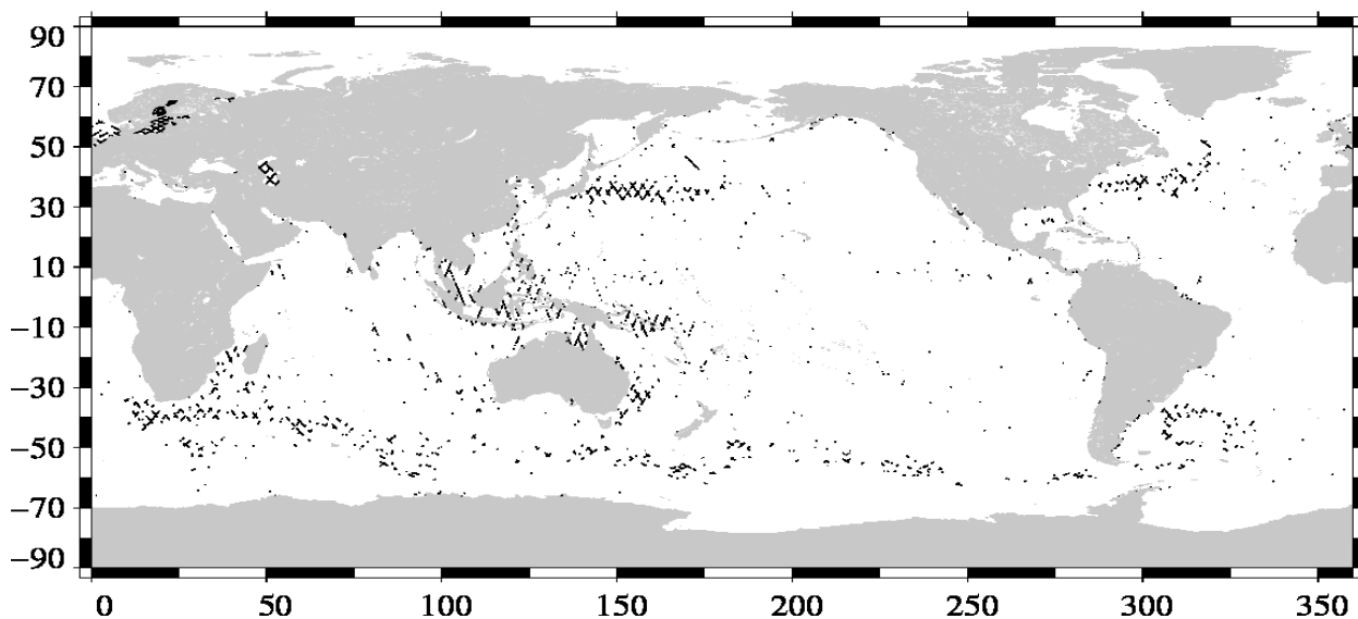
Valid data: (SSH – MSS) differences greater than 30 cm Jason-1 Cycle 369 (07/01/2012 / 17/01/2012)
