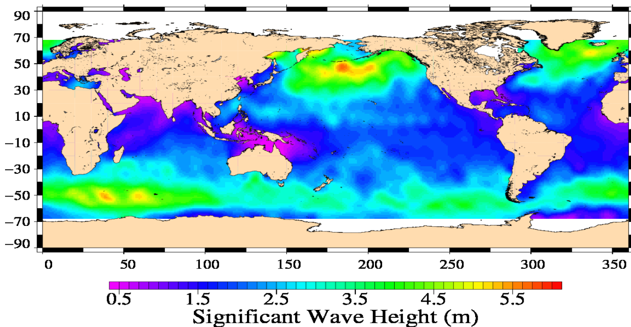
Jason-1 Cycle 369 07/01/2012 – 17/01/2012
