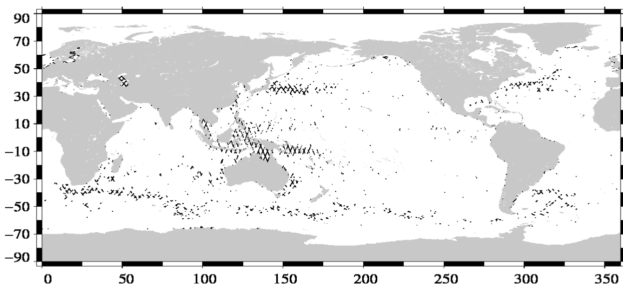
Valid data: (SSH – MSS) differences greater than 30 cm Jason-1 Cycle 371 (27/01/2012 / 05/02/2012)
