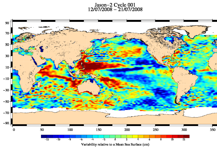
FIG. 19 – Sea level anomaly relative to MSS for cycle 001.
