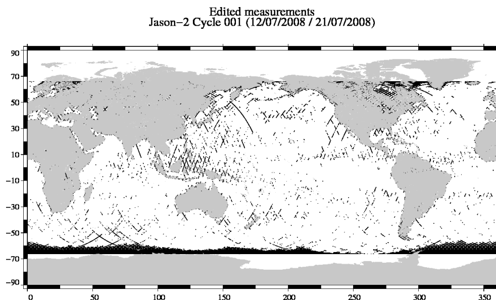
FIG. 2 – Edited measurements for cycle 001.
