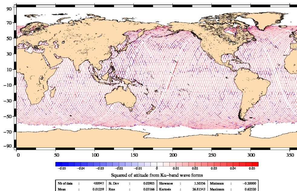
FIG. 4 – Apparent squared mispointing from waveforms for cycle 001.
