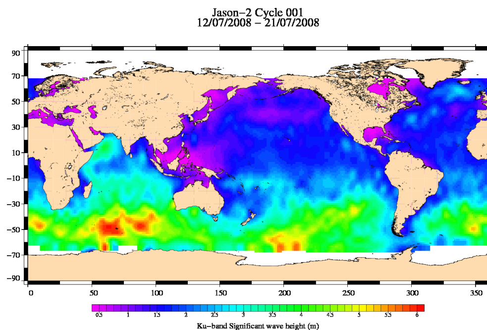
FIG. 6 – Significant wave height for cycle 001.
