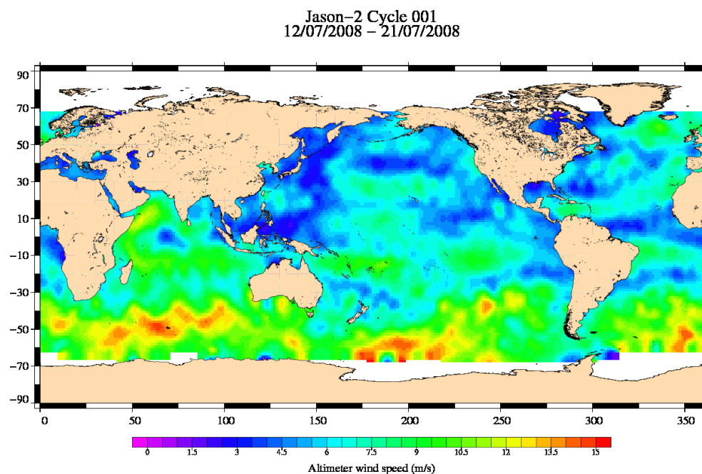
FIG. 10 – Altimeter wind speed for cycle 001.
