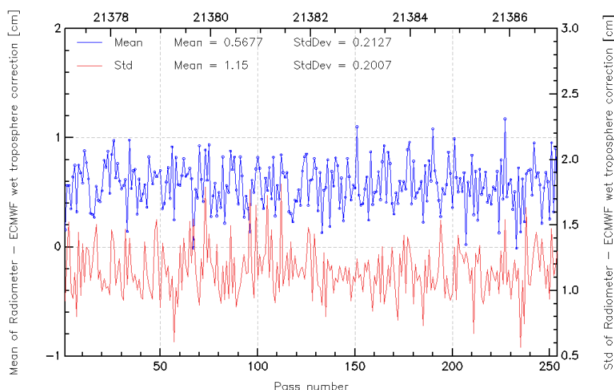
FIG. 12 – Pass monitoring of wet troposphere differences between radiometer and ECMWF model for Jason-2 cycle 001.
