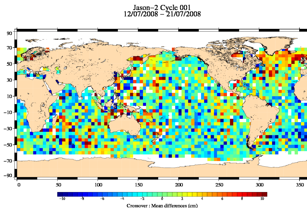
FIG. 14 – Mean SSH at crossovers for cycle 001.
