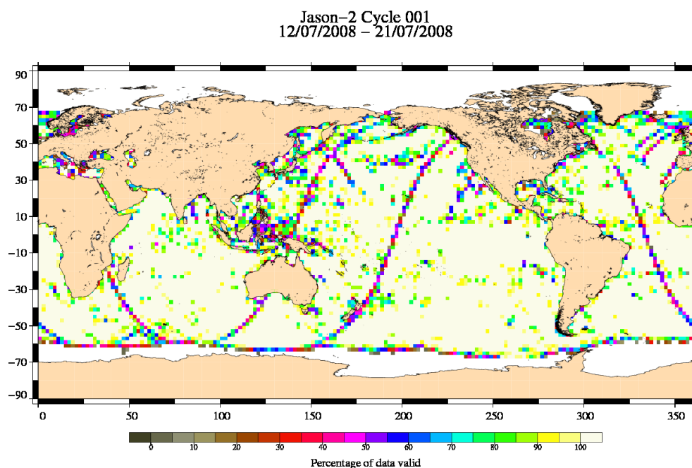
FIG. 3 – Percentage of valid measurements for cycle 001.
