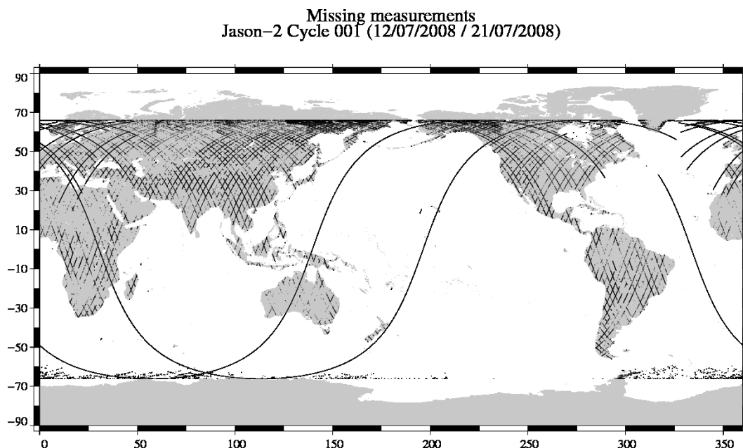
FIG. 1 – Missing measurements for cycle 001.
