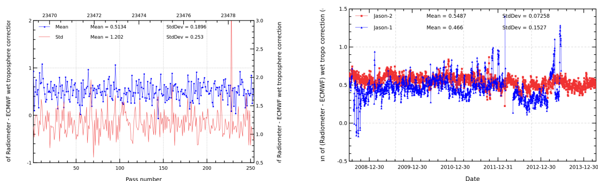
FIGURE 11 – Pass monitoring of wet troposphere differences between radiometer and ECMWF model for Jason-2 cycle 212 (left) and daily monitoring of wet troposphere differences between radiometer and ECMWF model (right).
