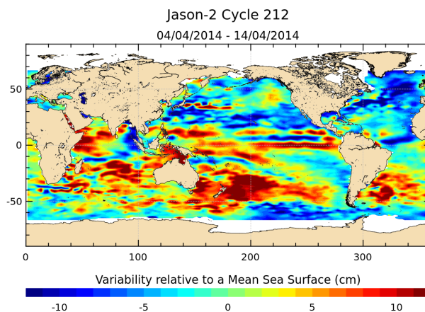
FIGURE 17 – Sea level anomaly relative to MSS for cycle 212.
