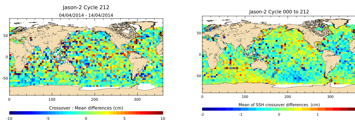
FIGURE 12 – Mean SSH at crossovers for cycle 212 (left) and over the whole Jason-2 period (right).
