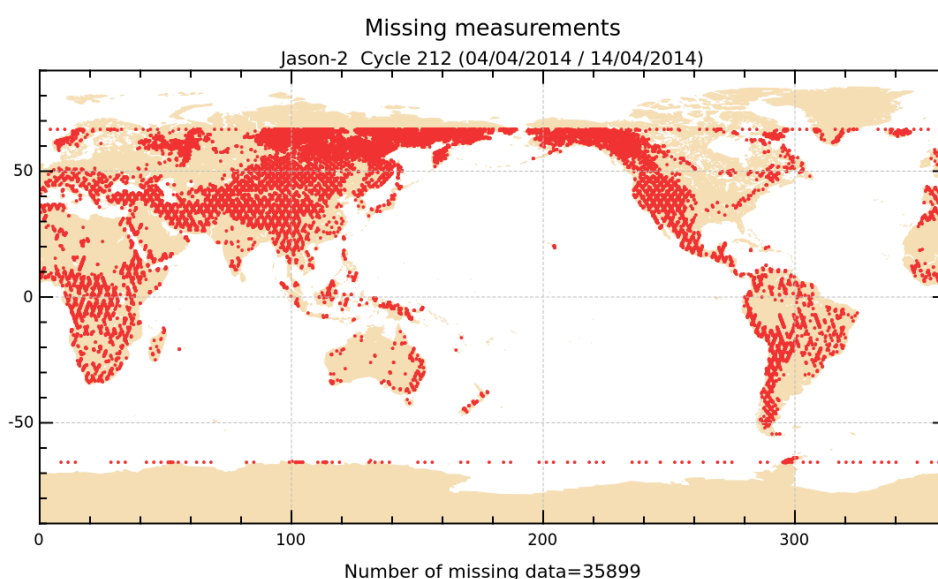
FIGURE 1 – Missing measurements for cycle 212.
