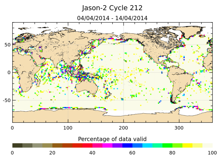
FIGURE 3 – Percentage of valid measurements for cycle 212.
