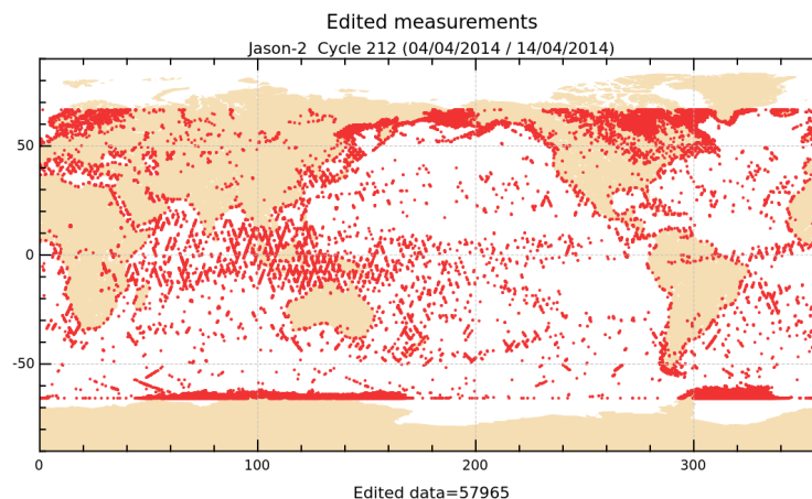
FIGURE 2 – Edited measurements for cycle 212.
