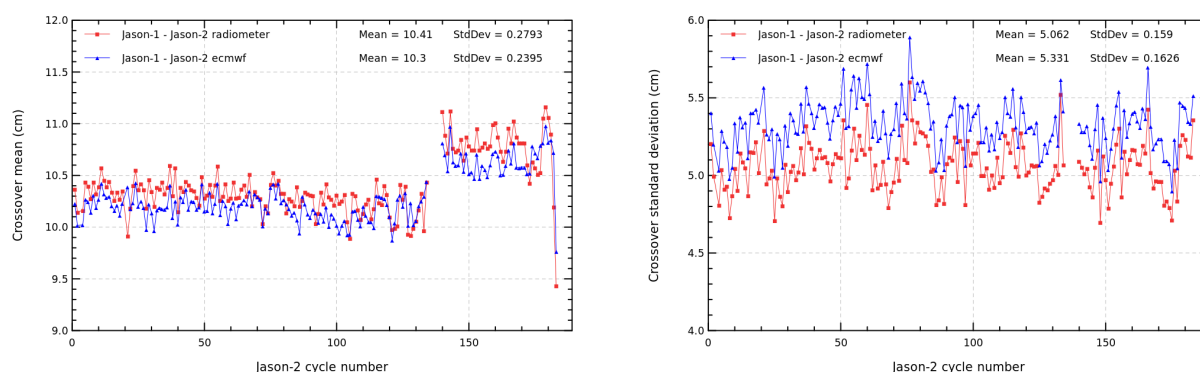
FIGURE 14 – Cyclic monitoring of mean (left) and standard deviation (right) of (Jason-1 – Jason-2) SSH differences at crossovers.
