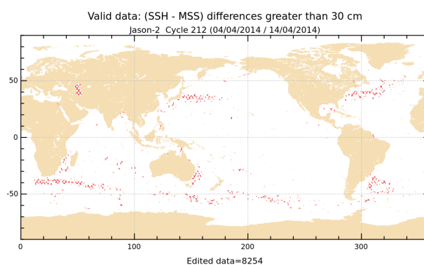
FIGURE 18 – Differences higher than a 30 cm threshold for cycle 212.
