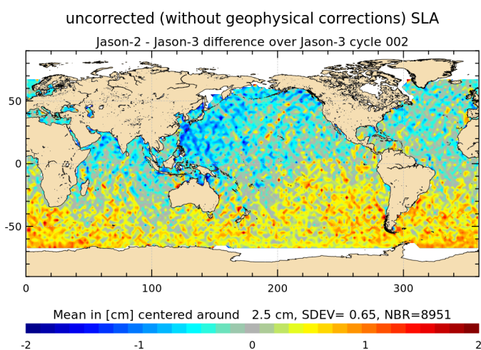
FIGURE 18 – Jason-2 – Jason-3 SLA differences (without corrections) for cycle 002.
