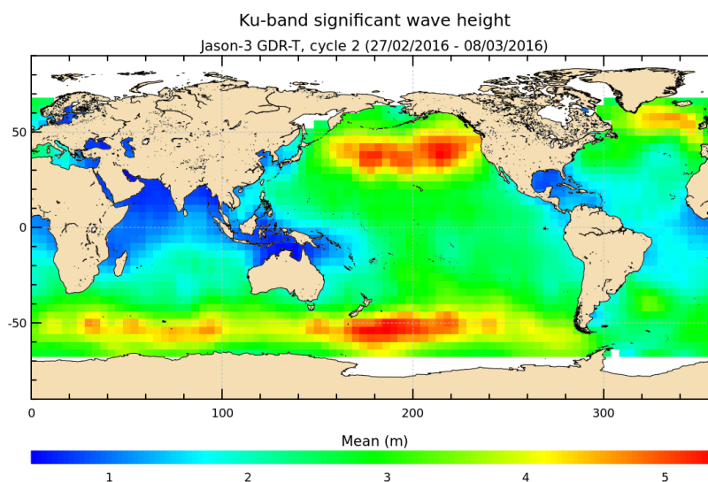
FIGURE 5 – Significant wave height for cycle 002.
