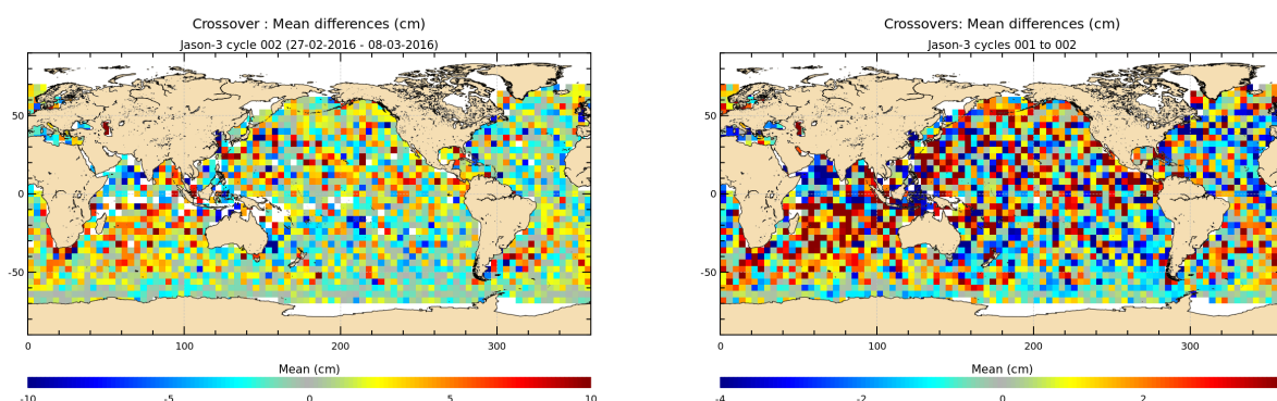
FIGURE 12 – Mean SSH at crossovers for cycle 002 (left) and over the whole Jason-3 period (right).
