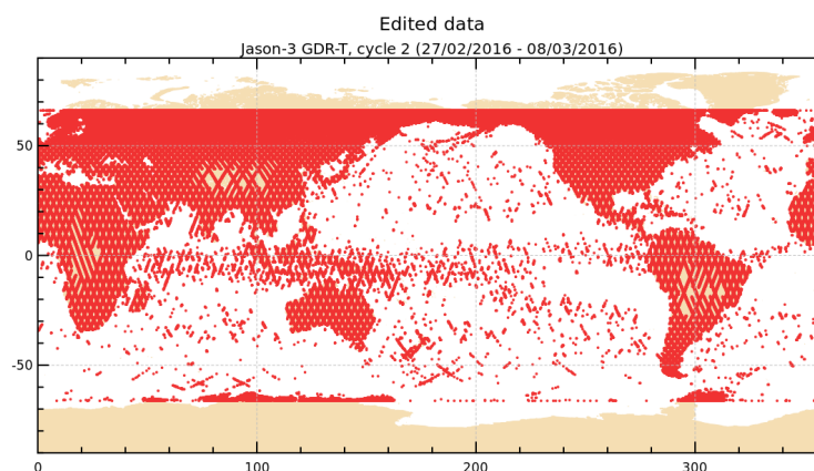
FIGURE 2 – Edited measurements for cycle 002.
