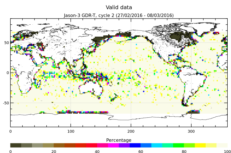
FIGURE 3 – Percentage of valid measurements for cycle 002.
