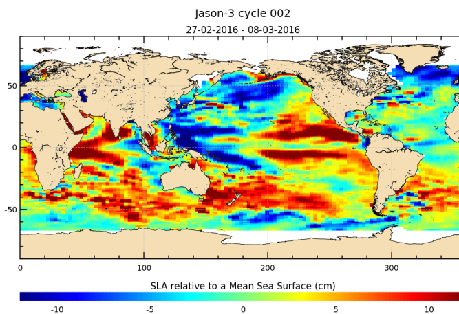
FIGURE 17 – Sea level anomaly relative to MSS for cycle 002.
