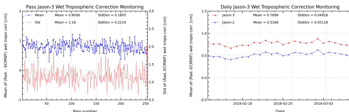
FIGURE 11 – Pass monitoring of wet troposphere differences between radiometer and ECMWF model for Jason-3 cycle 002 (left) and Jason-3 versus Jason-2 daily monitoring of wet troposphere differences between radiometer and ECMWF model (right).
