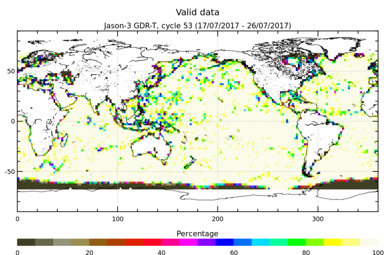
FIGURE 3 – Percentage of valid measurements for cycle 053.
