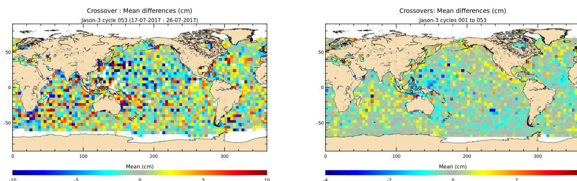
FIGURE 12 – Mean SSH at crossovers for cycle 053 (left) and over the whole Jason-3 period (right).
