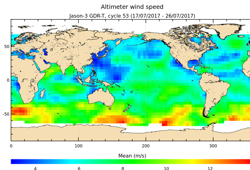
FIGURE 9 – Altimeter wind speed for cycle 053.
