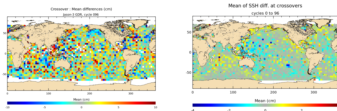
FIGURE 12 – Mean SSH at crossovers for cycle 096 (left) and over the whole Jason-3 period (right).
