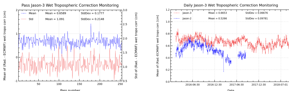
FIGURE 11 – Pass monitoring of wet troposphere differences between radiometer and ECMWF model for Jason-3 cycle 096 (left) and Jason-3 versus Jason-2 daily monitoring of wet troposphere differences between radiometer and ECMWF model (right).
