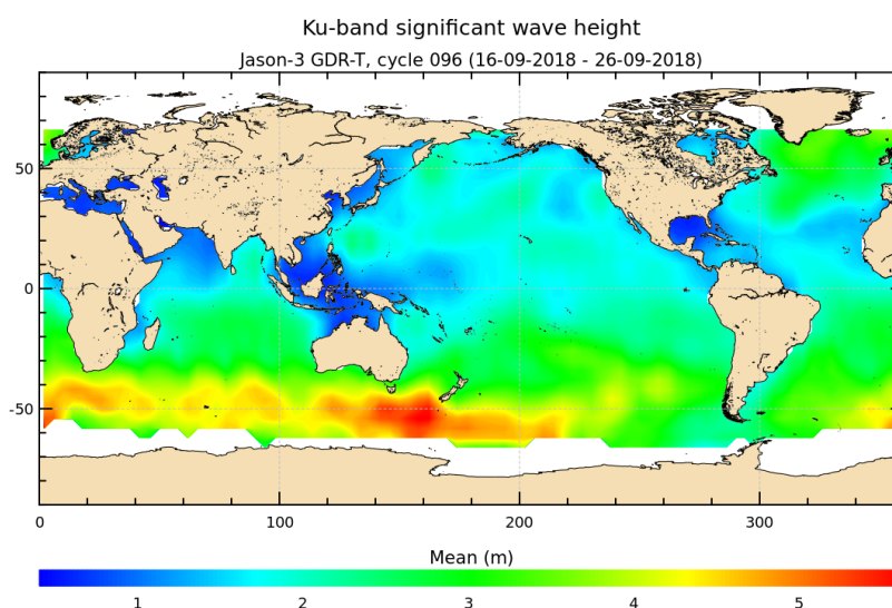
FIGURE 5 – Significant wave height for cycle 096.
