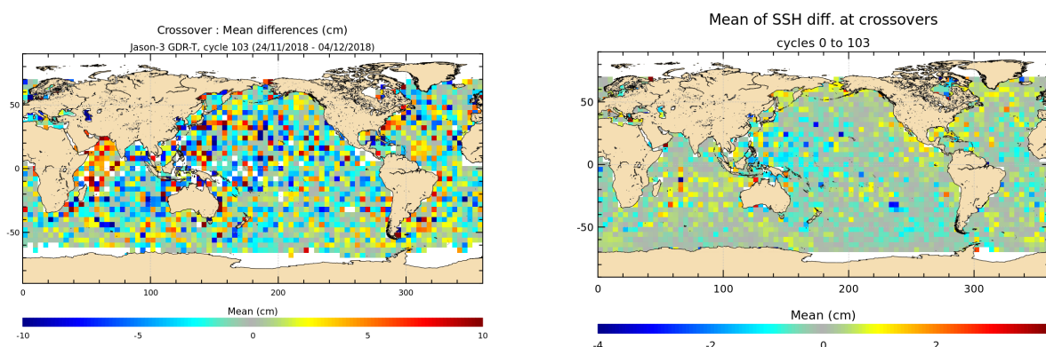
FIGURE 12 – Mean SSH at crossovers for cycle 103 (left) and over the whole Jason-3 period (right).
