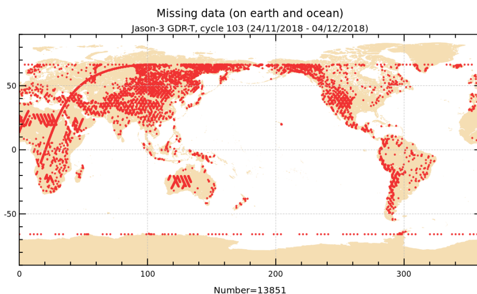
FIGURE 1 – Missing measurements for cycle 103.
