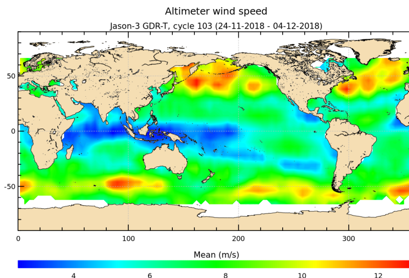
FIGURE 9 – Altimeter wind speed for cycle 103.
