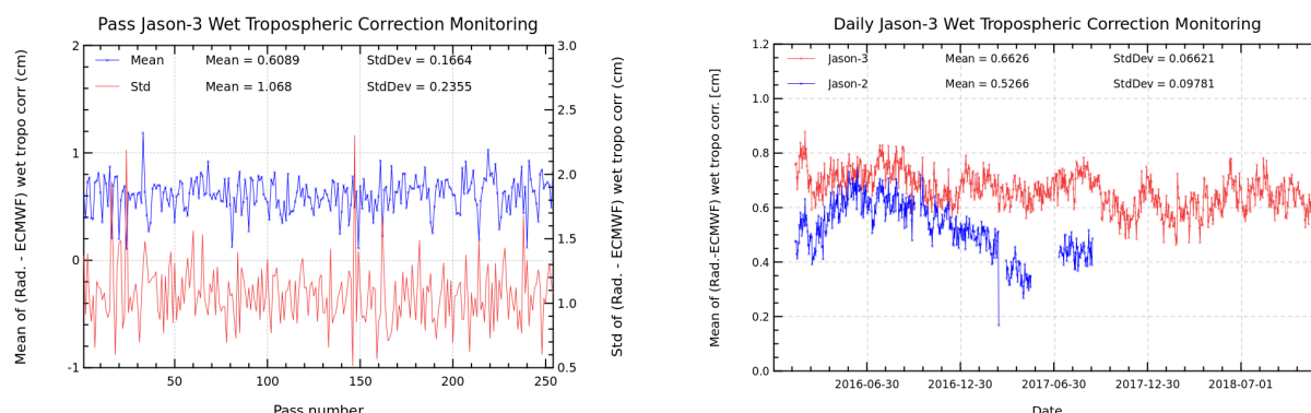
FIGURE 11 – Pass monitoring of wet troposphere differences between radiometer and ECMWF model for Jason-3 cycle 103 (left) and Jason-3 versus Jason-2 daily monitoring of wet troposphere differences between radiometer and ECMWF model (right).
