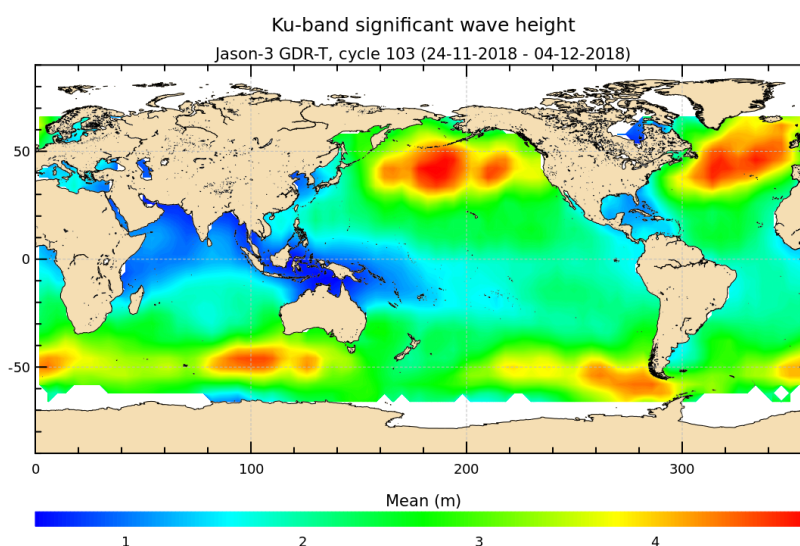
FIGURE 5 – Significant wave height for cycle 103.
