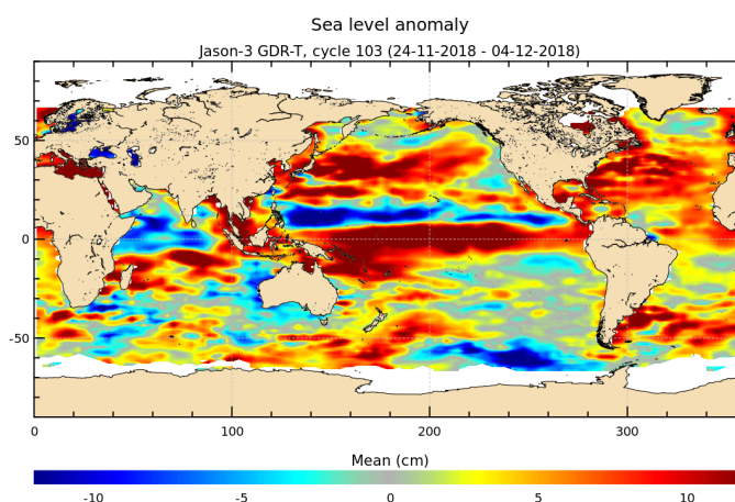
FIGURE 17 – Sea level anomaly relative to MSS for cycle 103.
