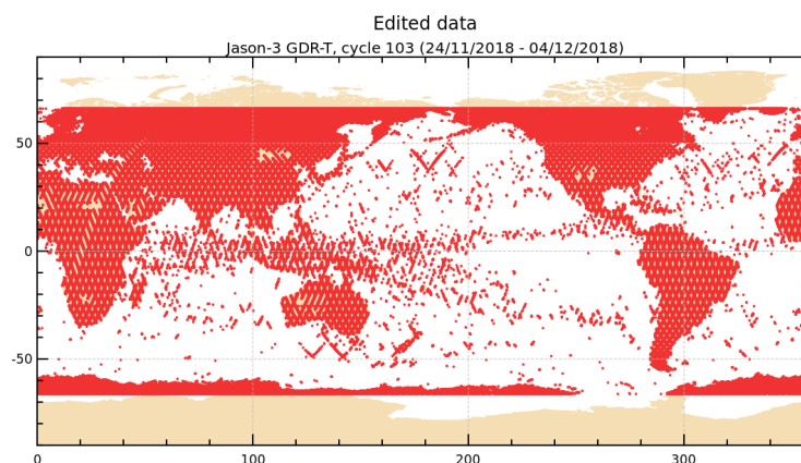
FIGURE 2 – Edited measurements for cycle 103.
