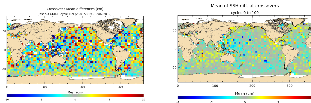
FIGURE 13 – Mean SSH at crossovers for cycle 109 (left) and over the whole Jason-3 period (right).
