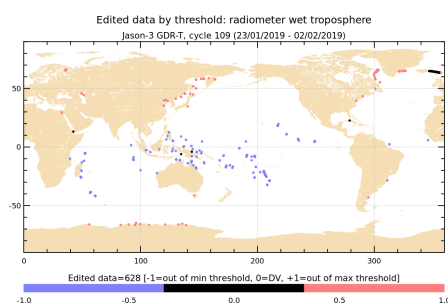
FIGURE 12 – Edited measurements by threshold for radiometer wet troposphere for cycle 109.
