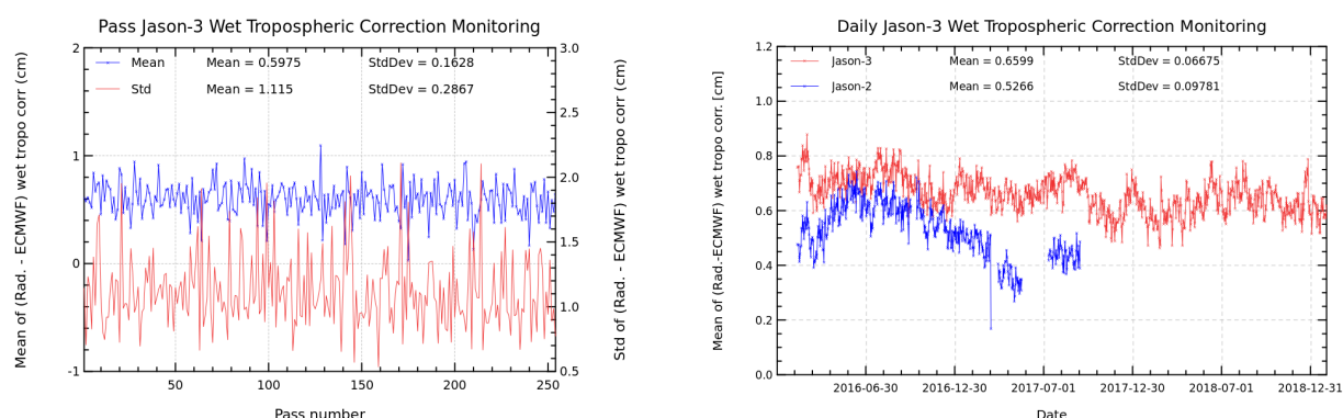
FIGURE 11 – Pass monitoring of wet troposphere differences between radiometer and ECMWF model for Jason-3 cycle 109 (left) and Jason-3 versus Jason-2 daily monitoring of wet troposphere differences between radiometer and ECMWF model (right).
