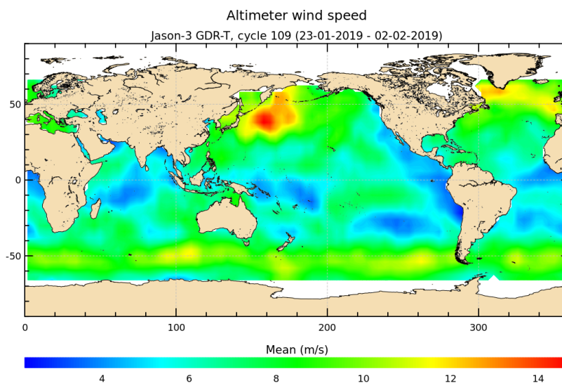
FIGURE 9 – Altimeter wind speed for cycle 109.
