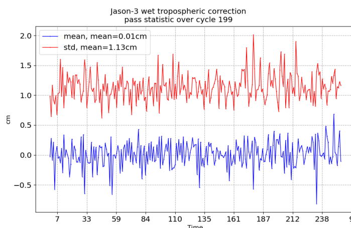
FIGURE 11 – Pass monitoring of wet troposphere differences between radiometer and ECMWF model for Jason-3 cycle 199
