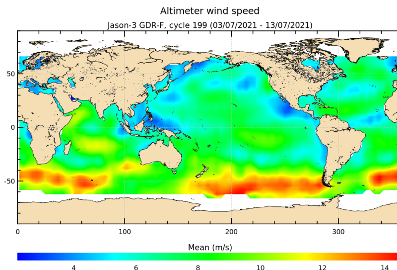
FIGURE 9 – Altimeter wind speed for cycle 199.
