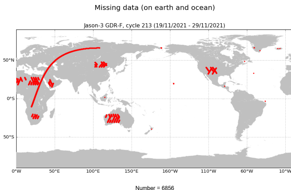
FIGURE 1 – Missing measurements for cycle 213.
