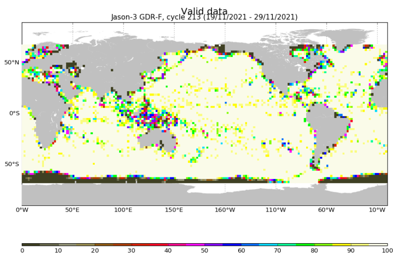
FIGURE 3 – Percentage of valid measurements for cycle 213.
