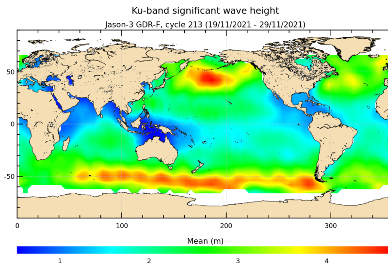
FIGURE 5 – Significant wave height for cycle 213.
