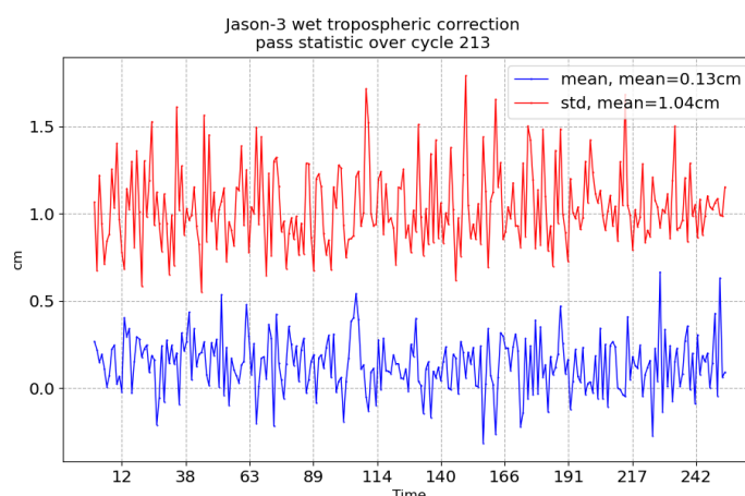
FIGURE 11 – Pass monitoring of wet troposphere differences between radiometer and ECMWF model for Jason-3 cycle 213
