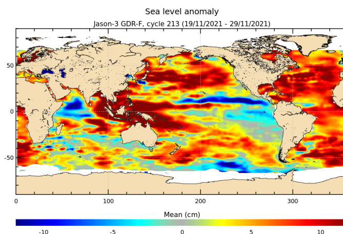
FIGURE 18 – Sea level anomaly relative to MSS for cycle 213.
