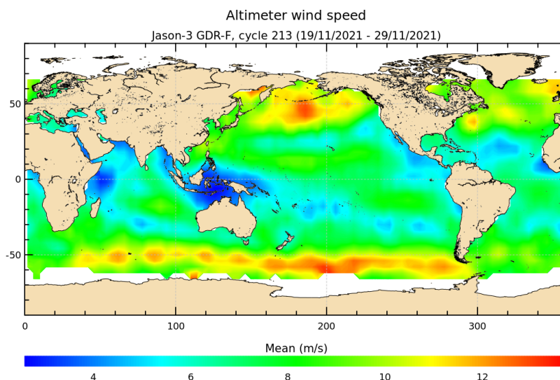
FIGURE 9 – Altimeter wind speed for cycle 213.
