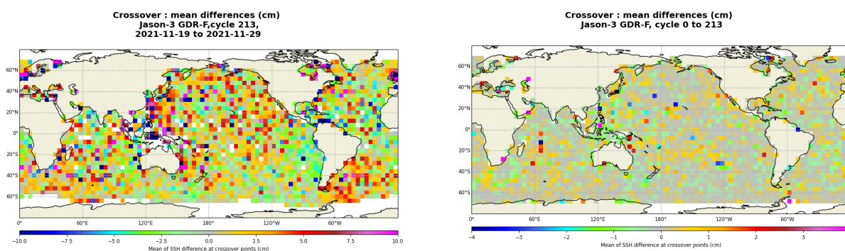
FIGURE 13 – Mean SSH at crossovers for cycle 213 (left) and over the whole Jason-3 period (right).
