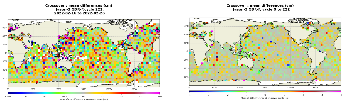
FIGURE 13 – Mean SSH at crossovers for cycle 222 (left) and over the whole Jason-3 period (right).
