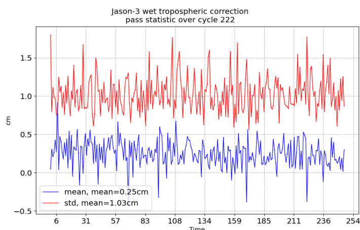
FIGURE 11 – Pass monitoring of wet troposphere differences between radiometer and ECMWF model for Jason-3 cycle 222
