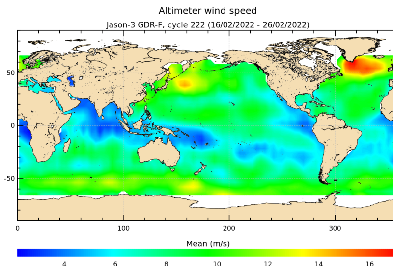
FIGURE 9 – Altimeter wind speed for cycle 222.
