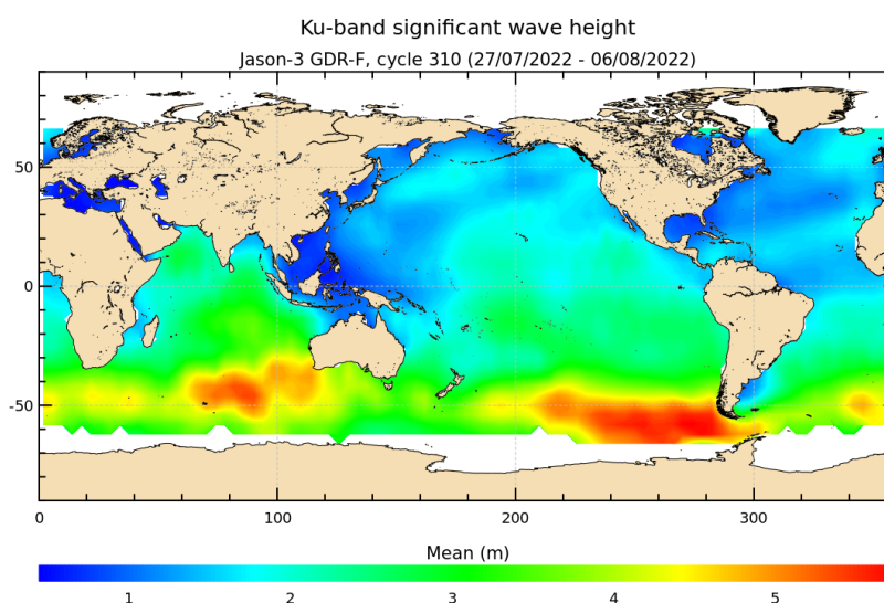
FIGURE 5 – Significant wave height for cycle 310.
