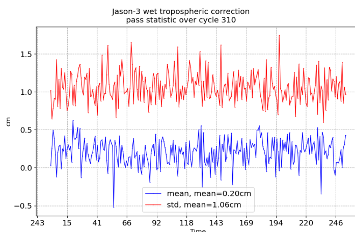
FIGURE 11 – Pass monitoring of wet troposphere differences between radiometer and ECMWF model for Jason-3 cycle 310
