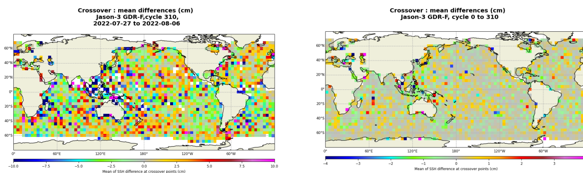
FIGURE 13 – Mean SSH at crossovers for cycle 310 (left) and over the whole Jason-3 period (right).
