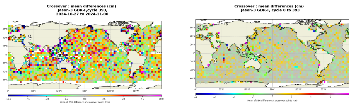
FIGURE 13 – Mean SSH at crossovers for cycle 393 (left) and over the whole Jason-3 period (right).
