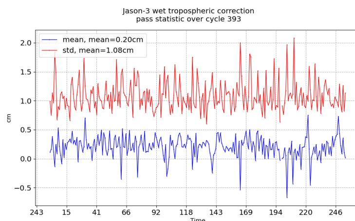
FIGURE 11 – Pass monitoring of wet troposphere differences between radiometer and ECMWF model for Jason-3 cycle 393
