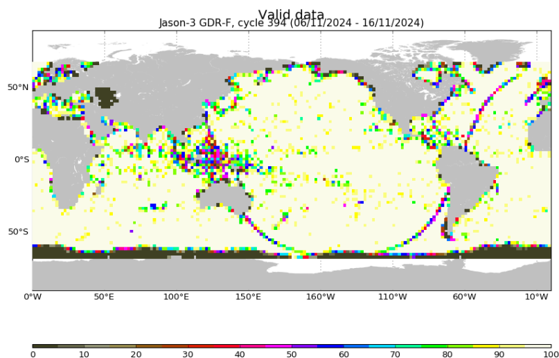
FIGURE 3 – Percentage of valid measurements for cycle 394.
