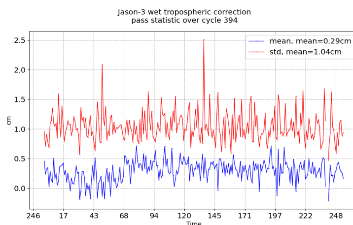
FIGURE 11 – Pass monitoring of wet troposphere differences between radiometer and ECMWF model for Jason-3 cycle 394
