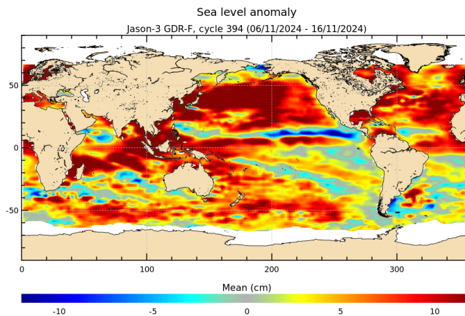
FIGURE 18 – Sea level anomaly relative to MSS for cycle 394.
