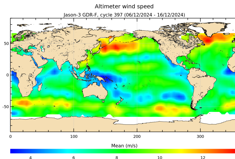
FIGURE 9 – Altimeter wind speed for cycle 397.
