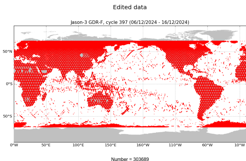
FIGURE 2 – Edited measurements for cycle 397.
