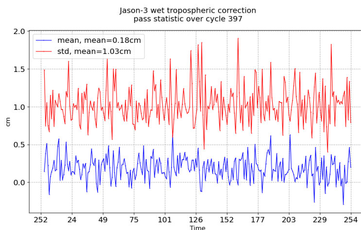
FIGURE 11 – Pass monitoring of wet troposphere differences between radiometer and ECMWF model for Jason-3 cycle 397
