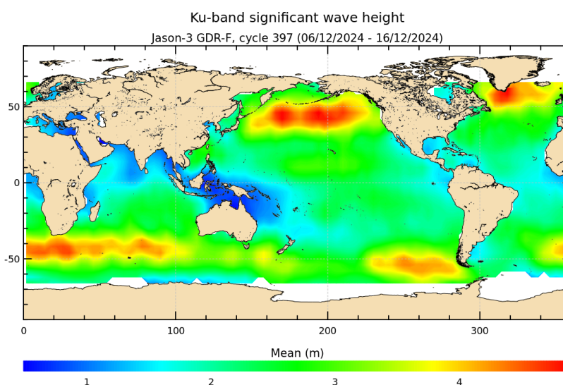
FIGURE 5 – Significant wave height for cycle 397.
