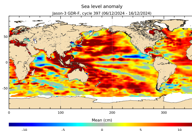
FIGURE 18 – Sea level anomaly relative to MSS for cycle 397.
