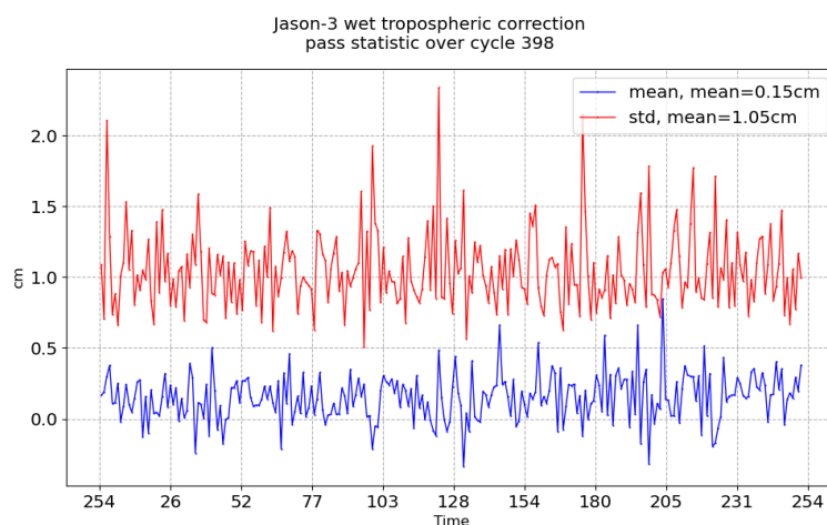
FIGURE 11 – Pass monitoring of wet troposphere differences between radiometer and ECMWF model for Jason-3 cycle 398
