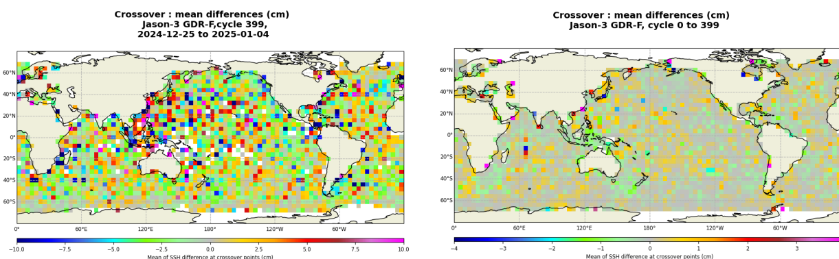
FIGURE 13 – Mean SSH at crossovers for cycle 399 (left) and over the whole Jason-3 period (right).
