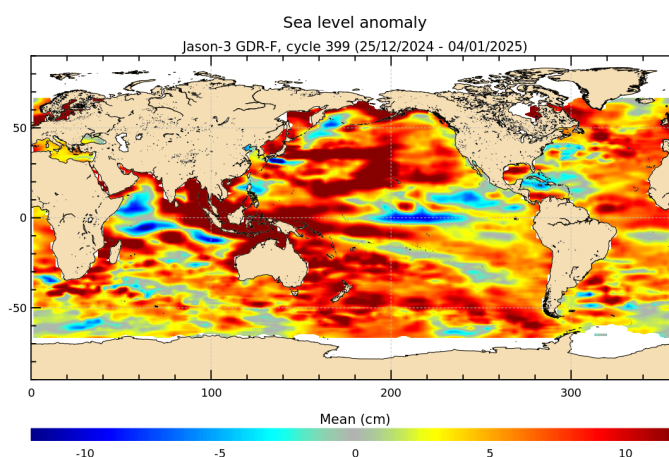
FIGURE 18 – Sea level anomaly relative to MSS for cycle 399.
