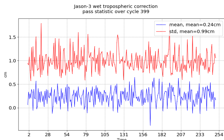
FIGURE 11 – Pass monitoring of wet troposphere differences between radiometer and ECMWF model for Jason-3 cycle 399
