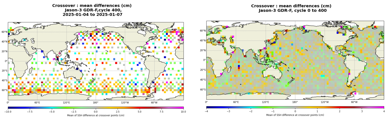
FIGURE 13 – Mean SSH at crossovers for cycle 400 (left) and over the whole Jason-3 period (right).
