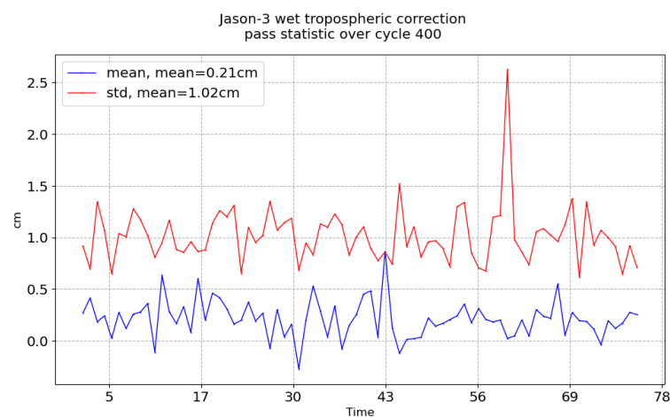
FIGURE 11 – Pass monitoring of wet troposphere differences between radiometer and ECMWF model for Jason-3 cycle 400
