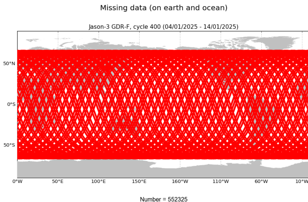
FIGURE 1 – Missing measurements for cycle 400.
