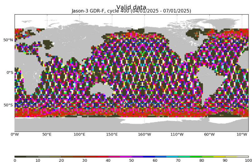
FIGURE 3 – Percentage of valid measurements for cycle 400.
