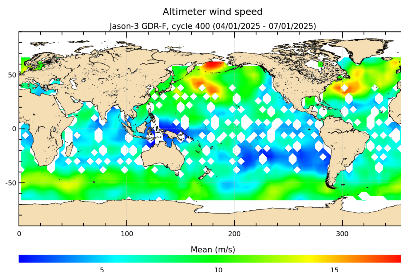
FIGURE 9 – Altimeter wind speed for cycle 400.
