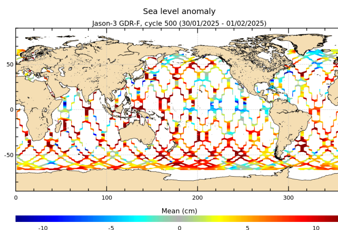
FIGURE 18 – Sea level anomaly relative to MSS for cycle 500.
