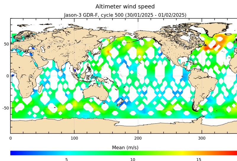
FIGURE 9 – Altimeter wind speed for cycle 500.
