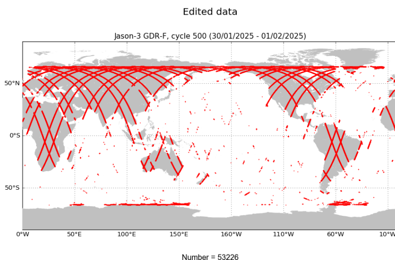
FIGURE 2 – Edited measurements for cycle 500.
