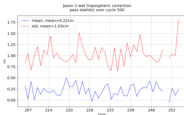
FIGURE 11 – Pass monitoring of wet troposphere differences between radiometer and ECMWF model for Jason-3 cycle 500
