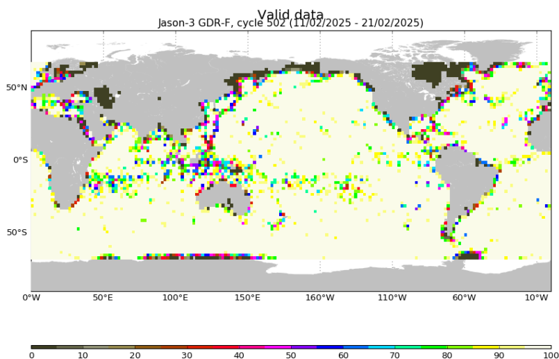
FIGURE 3 – Percentage of valid measurements for cycle 502.
