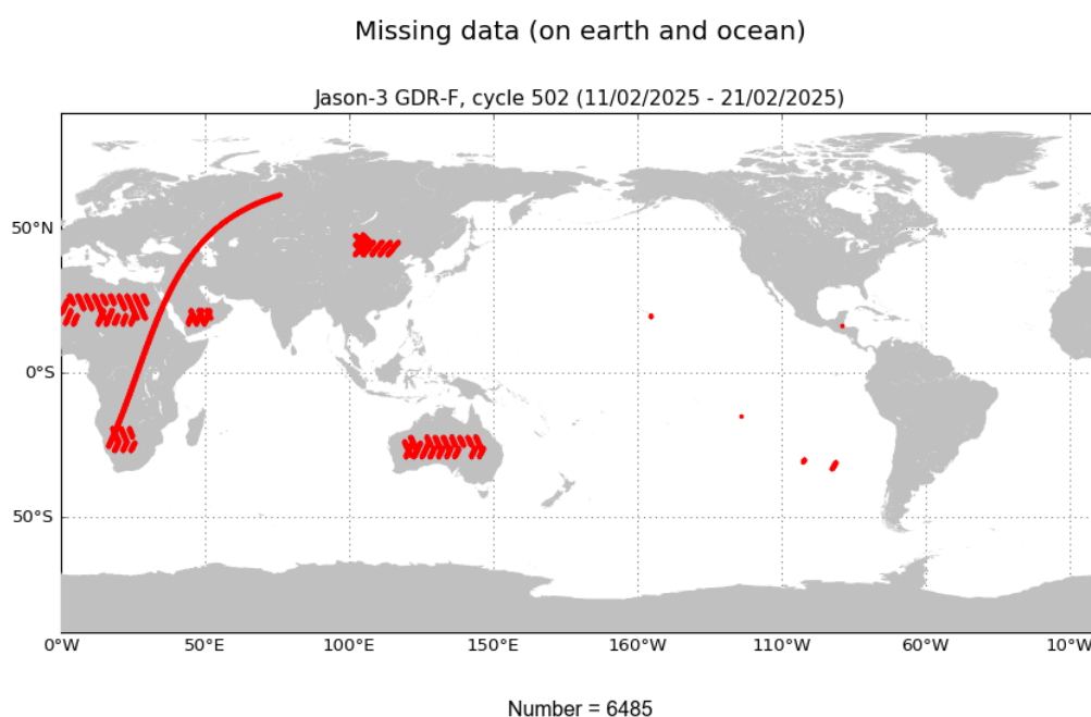
FIGURE 1 – Missing measurements for cycle 502.
