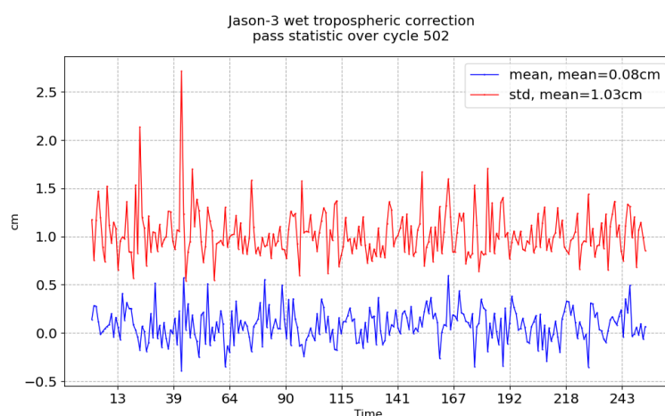
FIGURE 11 – Pass monitoring of wet troposphere differences between radiometer and ECMWF model for Jason-3 cycle 502
