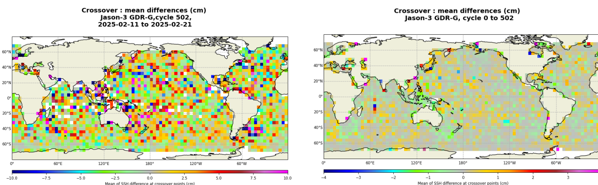
FIGURE 13 – Mean SSH at crossovers for cycle 502 (left) and over the whole Jason-3 period (right).
