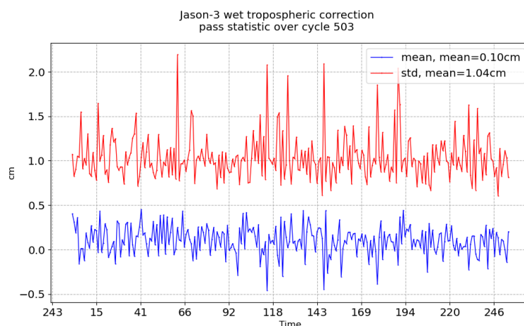
FIGURE 11 – Pass monitoring of wet troposphere differences between radiometer and ECMWF model for Jason-3 cycle 503
