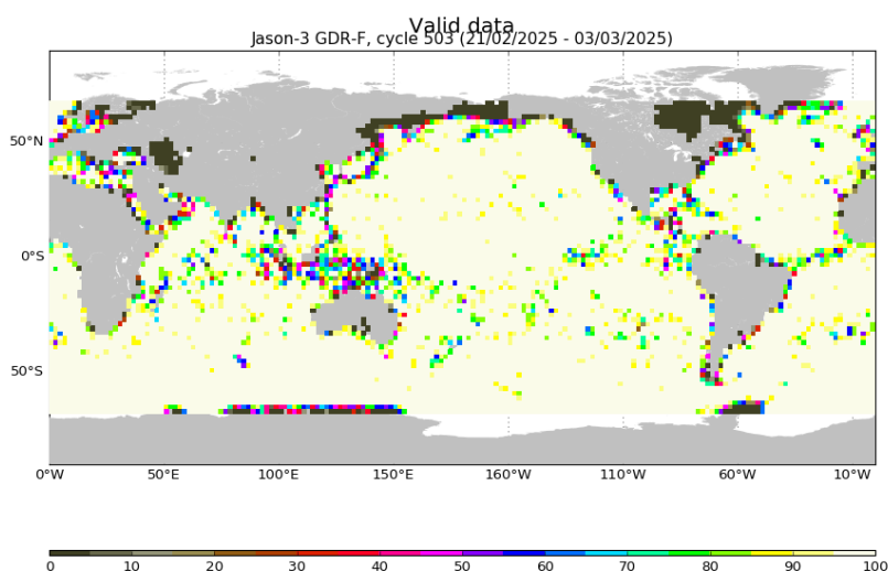
FIGURE 3 – Percentage of valid measurements for cycle 503.
