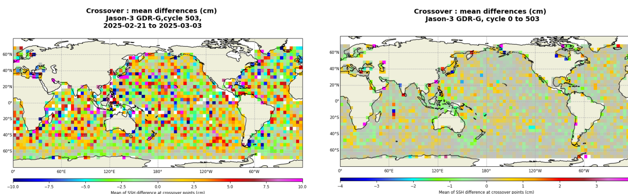
FIGURE 13 – Mean SSH at crossovers for cycle 503 (left) and over the whole Jason-3 period (right).
