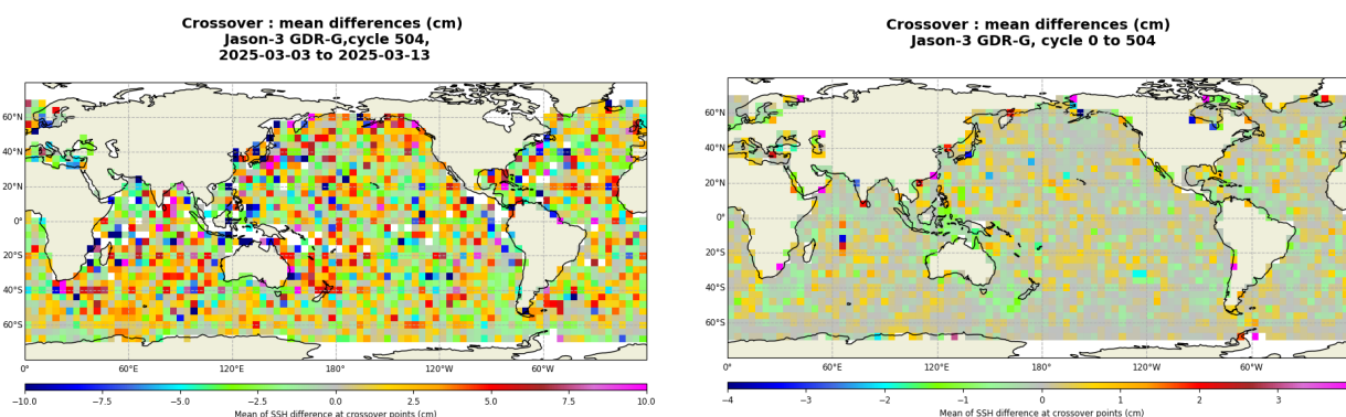
FIGURE 13 – Mean SSH at crossovers for cycle 504 (left) and over the whole Jason-3 period (right).
