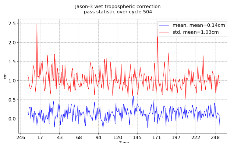
FIGURE 11 – Pass monitoring of wet troposphere differences between radiometer and ECMWF model for Jason-3 cycle 504
