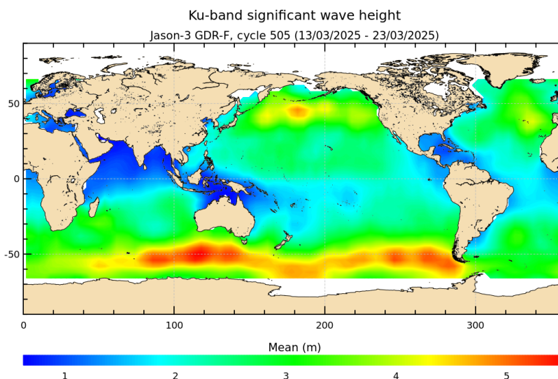
FIGURE 5 – Significant wave height for cycle 505.
