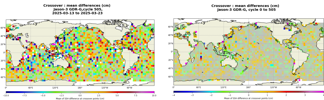
FIGURE 13 – Mean SSH at crossovers for cycle 505 (left) and over the whole Jason-3 period (right).
