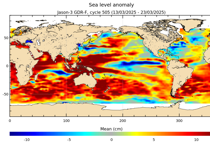
FIGURE 18 – Sea level anomaly relative to MSS for cycle 505.
