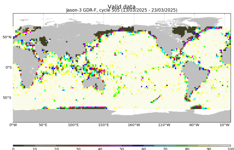
FIGURE 3 – Percentage of valid measurements for cycle 505.
