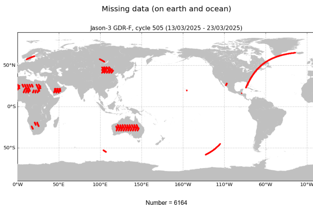
FIGURE 1 – Missing measurements for cycle 505.
