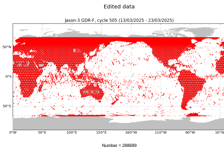
FIGURE 2 – Edited measurements for cycle 505.
