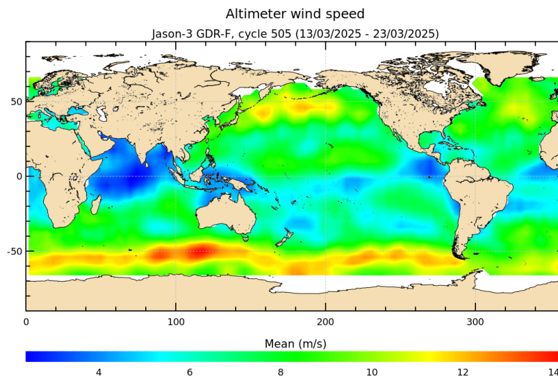
FIGURE 9 – Altimeter wind speed for cycle 505.
