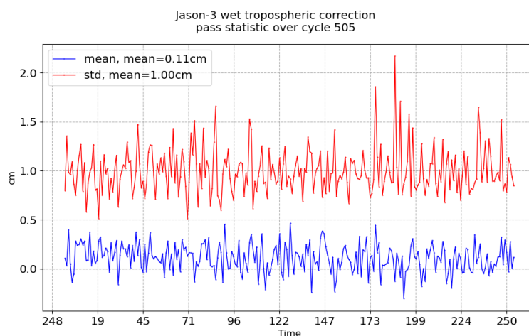
FIGURE 11 – Pass monitoring of wet troposphere differences between radiometer and ECMWF model for Jason-3 cycle 505
