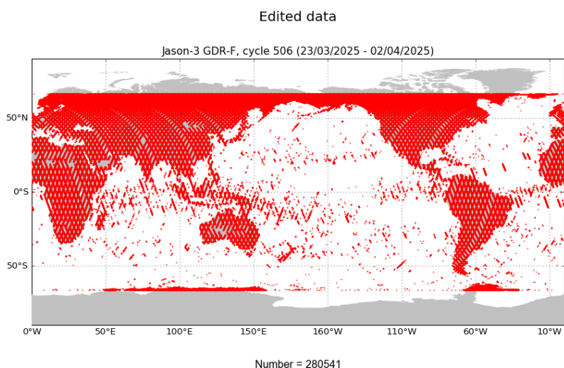
FIGURE 2 – Edited measurements for cycle 506.
