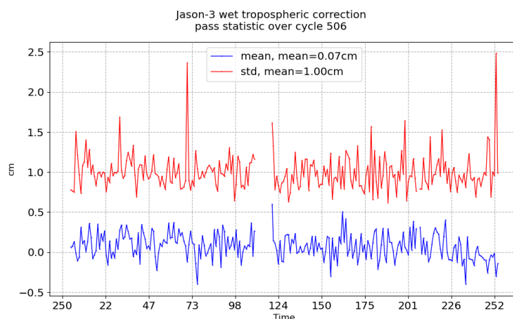
FIGURE 11 – Pass monitoring of wet troposphere differences between radiometer and ECMWF model for Jason-3 cycle 506
