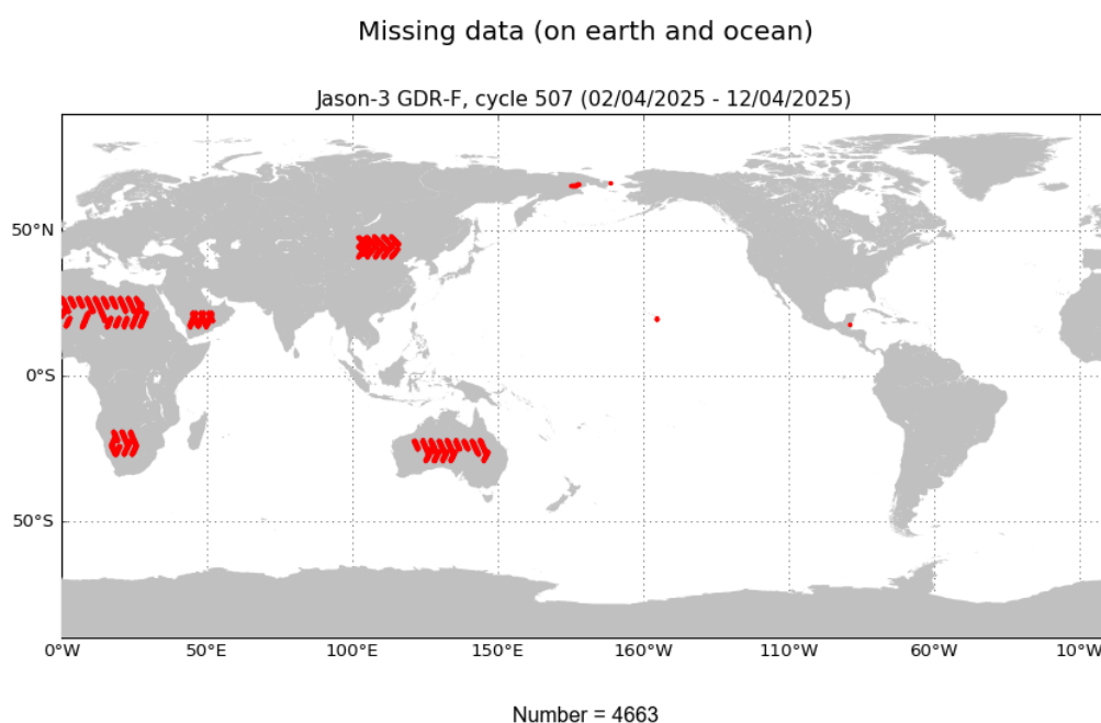
FIGURE 1 – Missing measurements for cycle 507.
