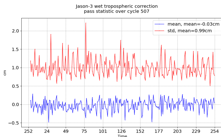
FIGURE 11 – Pass monitoring of wet troposphere differences between radiometer and ECMWF model for Jason-3 cycle 507
