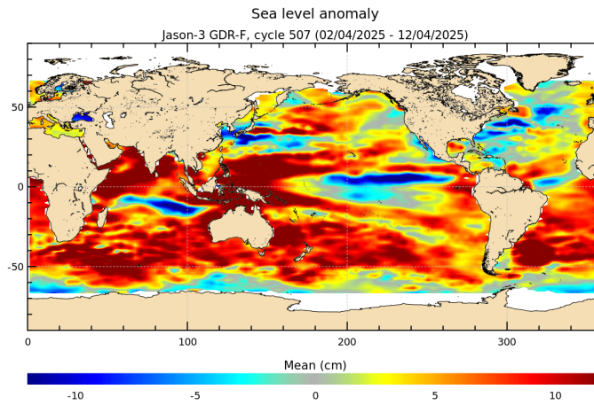
FIGURE 18 – Sea level anomaly relative to MSS for cycle 507.
