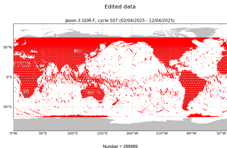
FIGURE 2 – Edited measurements for cycle 507.
