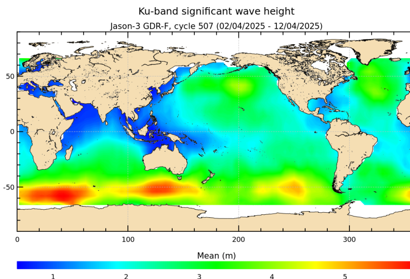
FIGURE 5 – Significant wave height for cycle 507.
