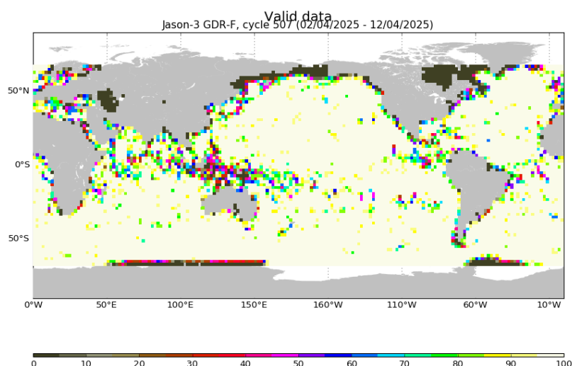
FIGURE 3 – Percentage of valid measurements for cycle 507.
