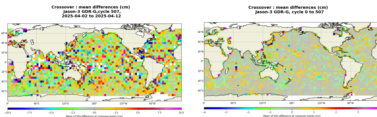
FIGURE 13 – Mean SSH at crossovers for cycle 507 (left) and over the whole Jason-3 period (right).
