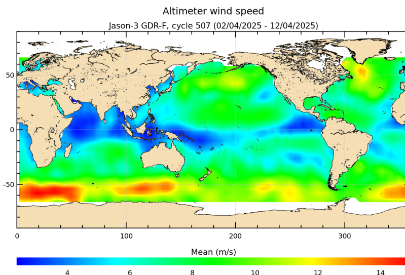
FIGURE 9 – Altimeter wind speed for cycle 507.
