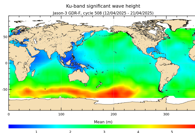
FIGURE 5 – Significant wave height for cycle 508.
