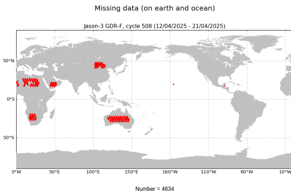
FIGURE 1 – Missing measurements for cycle 508.
