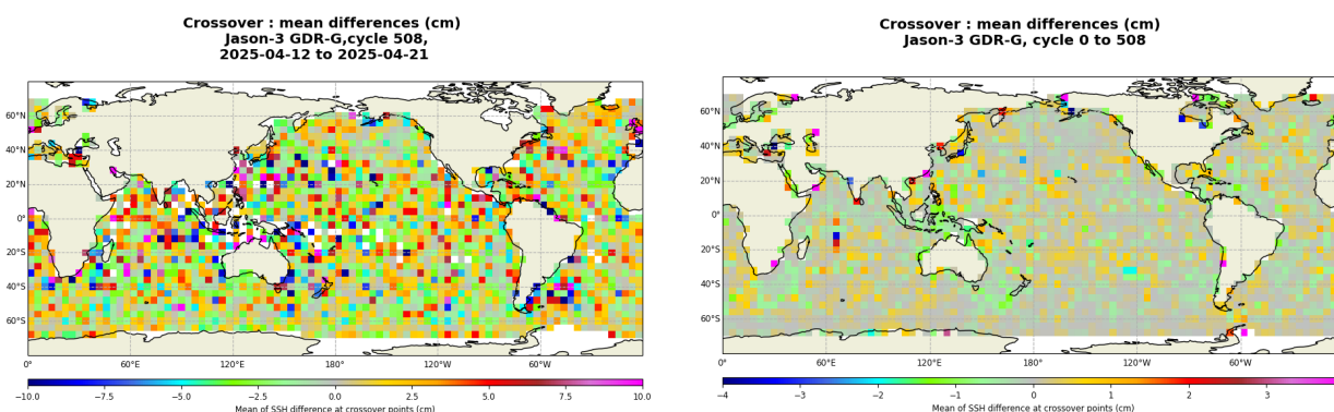
FIGURE 13 – Mean SSH at crossovers for cycle 508 (left) and over the whole Jason-3 period (right).
