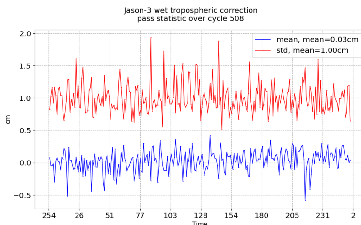
FIGURE 11 – Pass monitoring of wet troposphere differences between radiometer and ECMWF model for Jason-3 cycle 508
