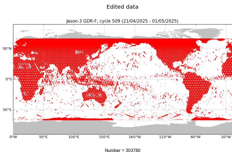
FIGURE 2 – Edited measurements for cycle 509.
