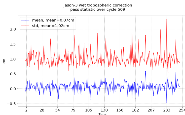
FIGURE 11 – Pass monitoring of wet troposphere differences between radiometer and ECMWF model for Jason-3 cycle 509
