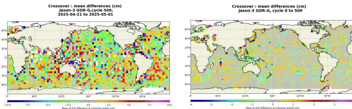
FIGURE 13 – Mean SSH at crossovers for cycle 509 (left) and over the whole Jason-3 period (right).
