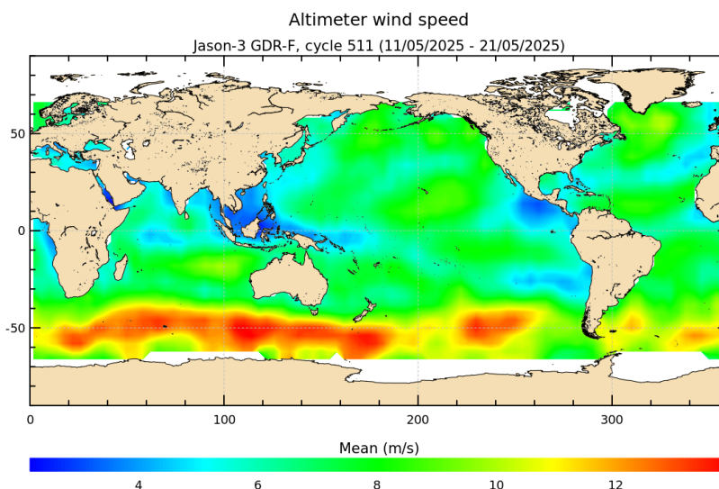
FIGURE 9 – Altimeter wind speed for cycle 511.
