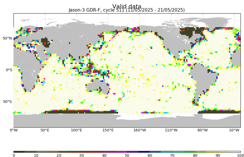
FIGURE 3 – Percentage of valid measurements for cycle 511.
