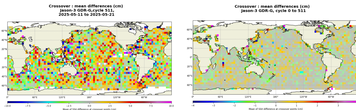
FIGURE 13 – Mean SSH at crossovers for cycle 511 (left) and over the whole Jason-3 period (right).
