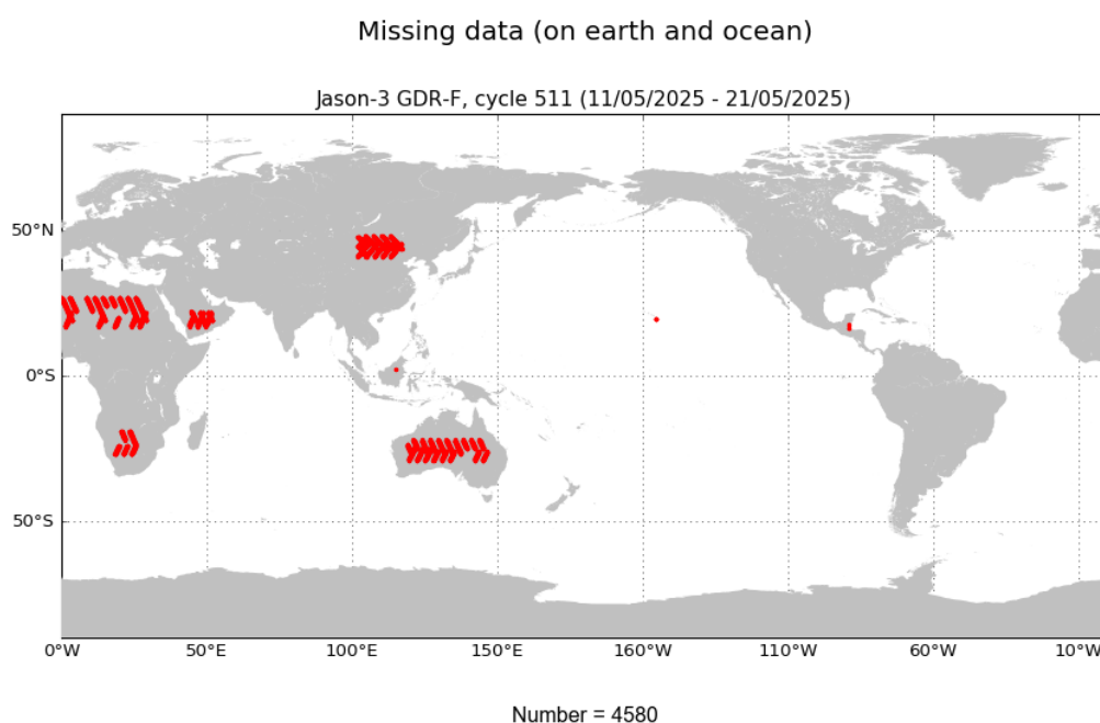
FIGURE 1 – Missing measurements for cycle 511.
