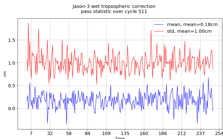
FIGURE 11 – Pass monitoring of wet troposphere differences between radiometer and ECMWF model for Jason-3 cycle 511
