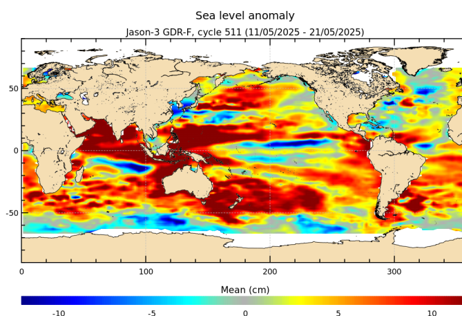
FIGURE 18 – Sea level anomaly relative to MSS for cycle 511.
