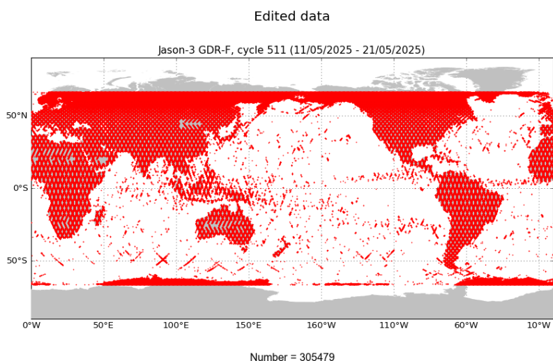
FIGURE 2 – Edited measurements for cycle 511.
