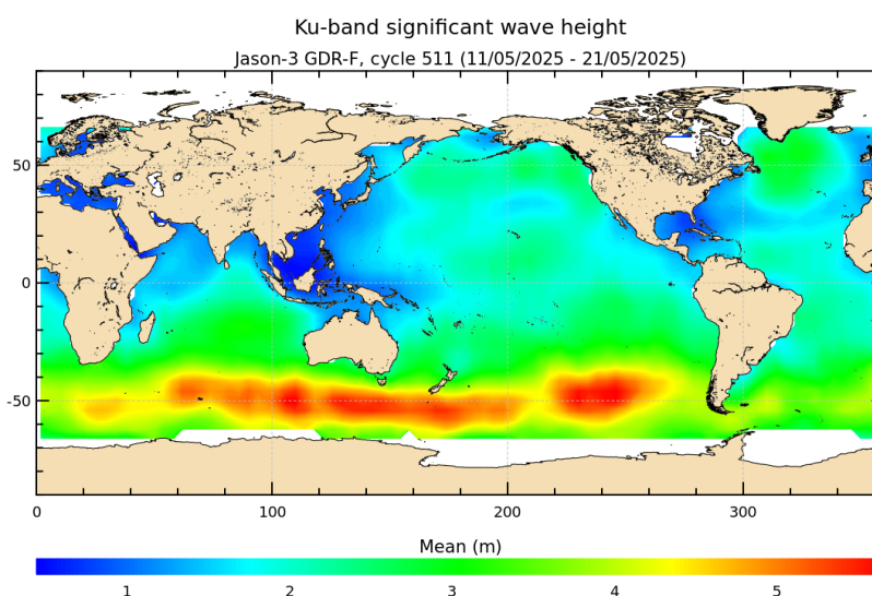
FIGURE 5 – Significant wave height for cycle 511.
