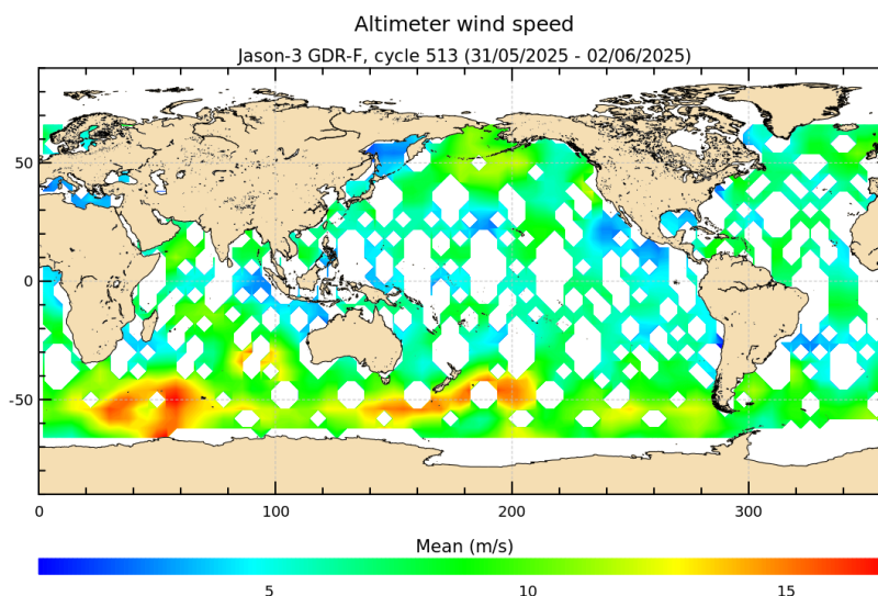
FIGURE 9 – Altimeter wind speed for cycle 513.
