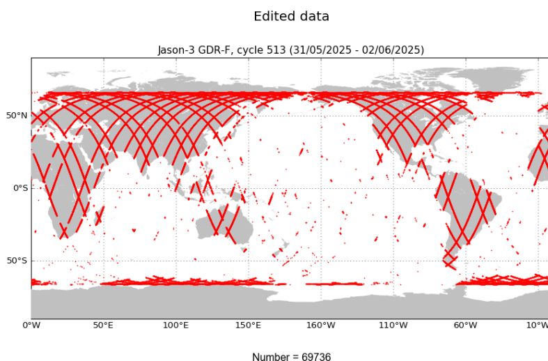
FIGURE 2 – Edited measurements for cycle 513.
