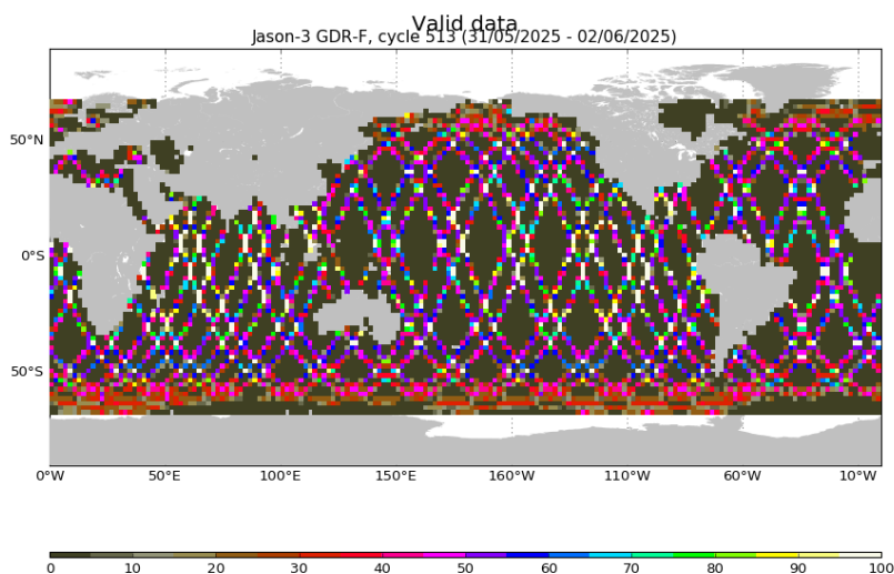
FIGURE 3 – Percentage of valid measurements for cycle 513.
