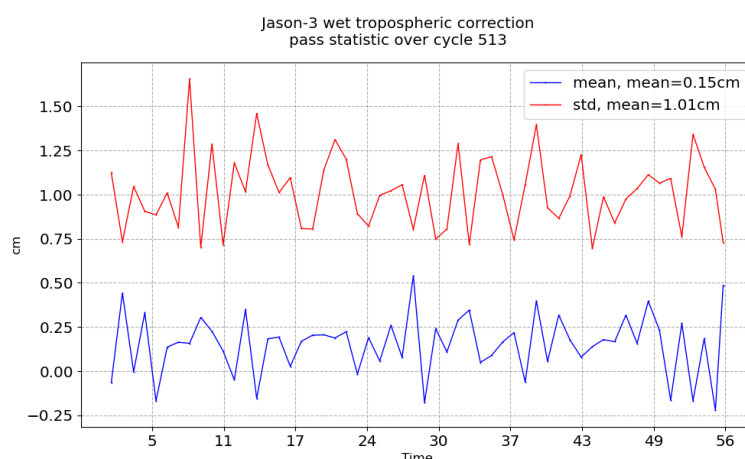
FIGURE 11 – Pass monitoring of wet troposphere differences between radiometer and ECMWF model for Jason-3 cycle 513
