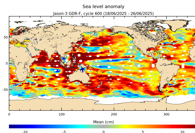
FIGURE 18 – Sea level anomaly relative to MSS for cycle 600.
