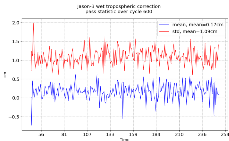
FIGURE 11 – Pass monitoring of wet troposphere differences between radiometer and ECMWF model for Jason-3 cycle 600
