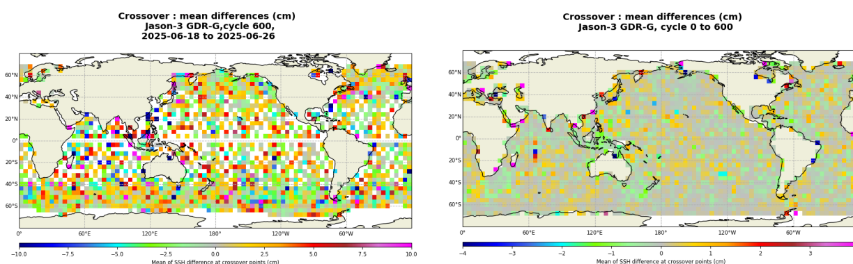
FIGURE 13 – Mean SSH at crossovers for cycle 600 (left) and over the whole Jason-3 period (right).
