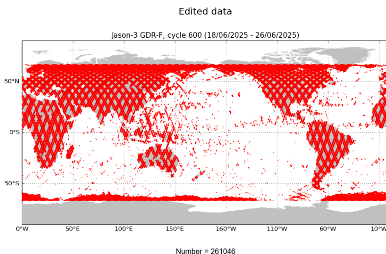
FIGURE 2 – Edited measurements for cycle 600.
