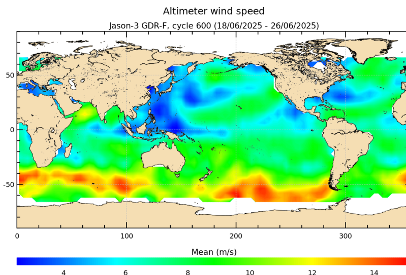
FIGURE 9 – Altimeter wind speed for cycle 600.
