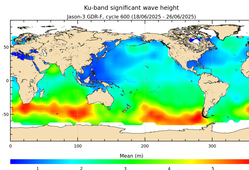
FIGURE 5 – Significant wave height for cycle 600.
