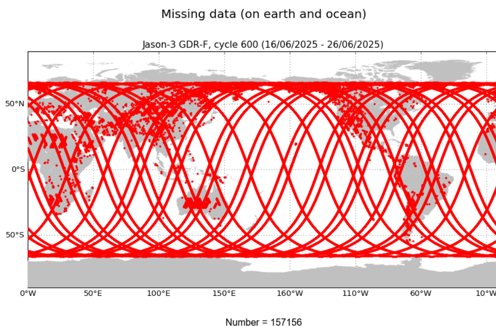
FIGURE 1 – Missing measurements for cycle 600.
