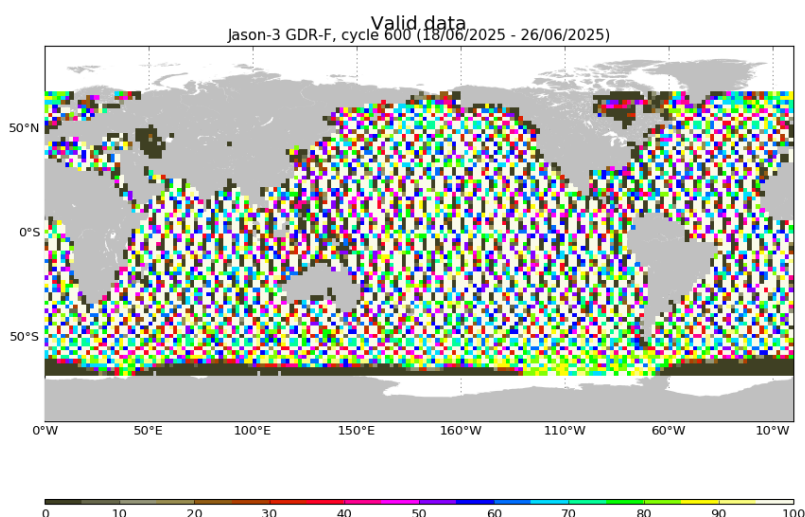
FIGURE 3 – Percentage of valid measurements for cycle 600.
