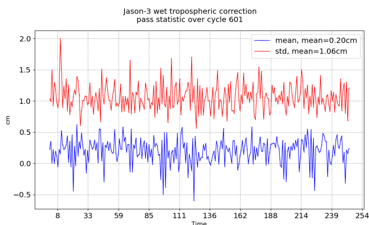
FIGURE 11 – Pass monitoring of wet troposphere differences between radiometer and ECMWF model for Jason-3 cycle 601
