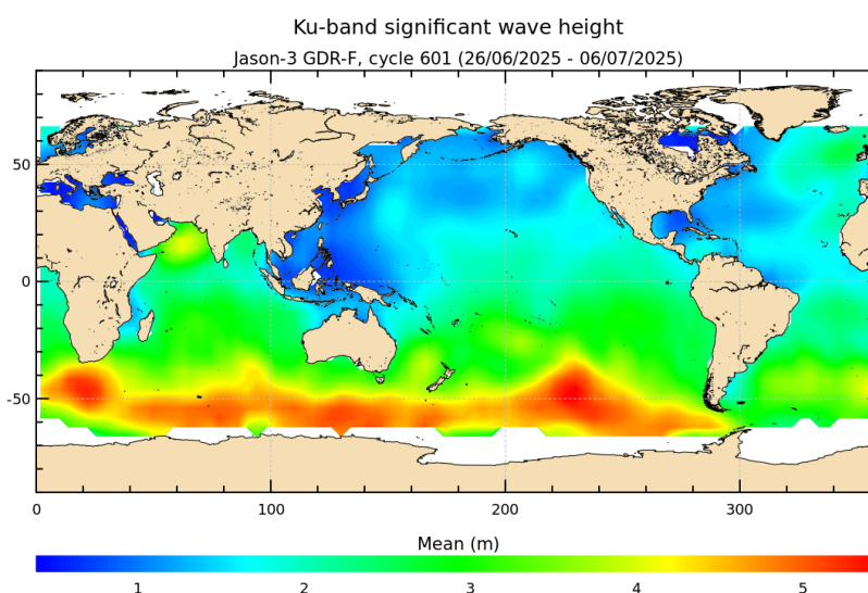
FIGURE 5 – Significant wave height for cycle 601.
