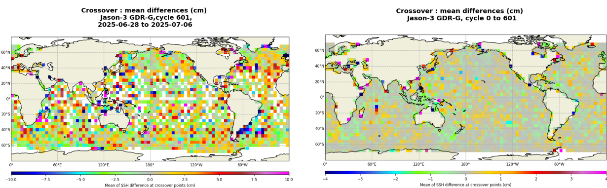
FIGURE 13 – Mean SSH at crossovers for cycle 601 (left) and over the whole Jason-3 period (right).
