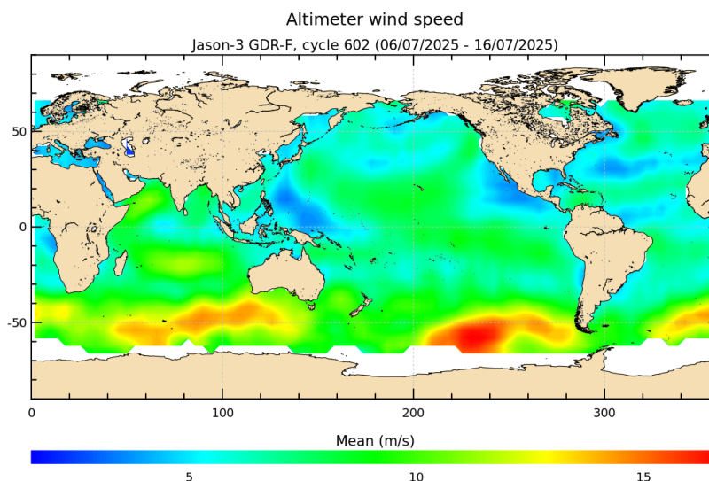
FIGURE 9 – Altimeter wind speed for cycle 602.
