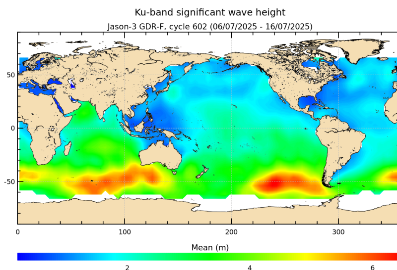
FIGURE 5 – Significant wave height for cycle 602.
