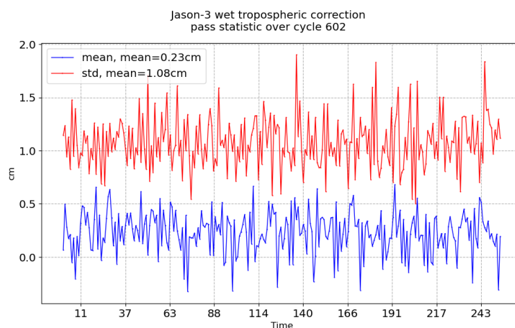
FIGURE 11 – Pass monitoring of wet troposphere differences between radiometer and ECMWF model for Jason-3 cycle 602
