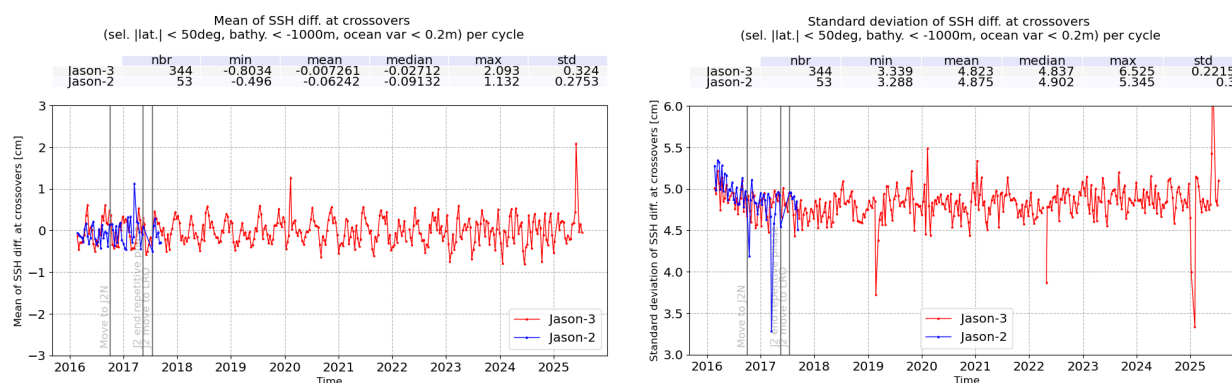
FIGURE 14 – Cyclic monitoring of mean (left) and standard deviation (right) of SSH differences at crossovers for Jason-3 and Jason-2.
