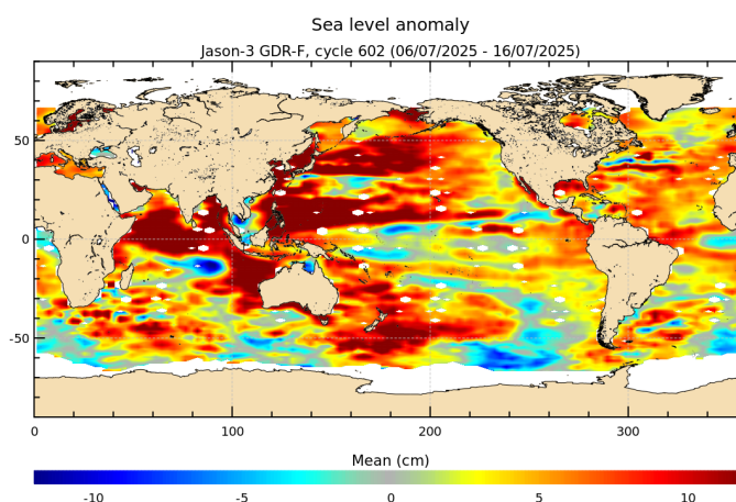
FIGURE 18 – Sea level anomaly relative to MSS for cycle 602.
