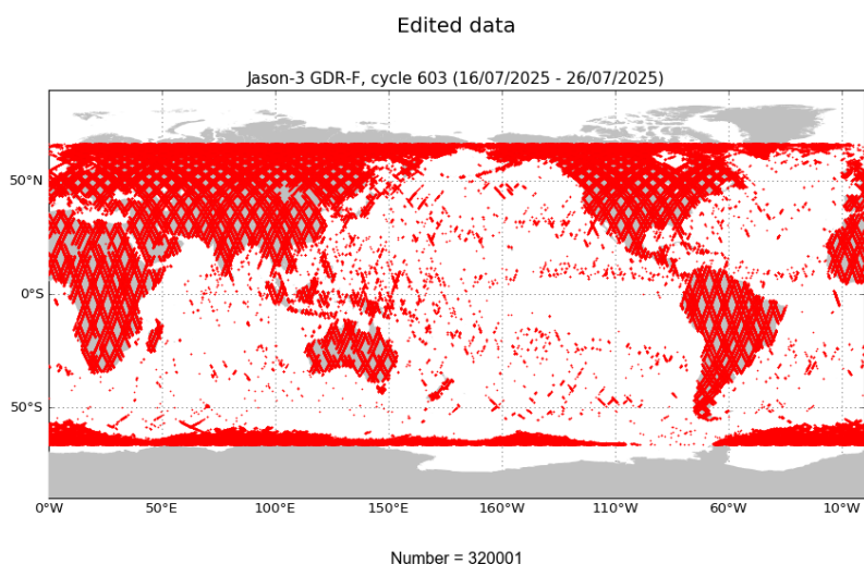
FIGURE 2 – Edited measurements for cycle 603.
