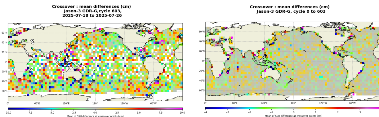
FIGURE 13 – Mean SSH at crossovers for cycle 603 (left) and over the whole Jason-3 period (right).
