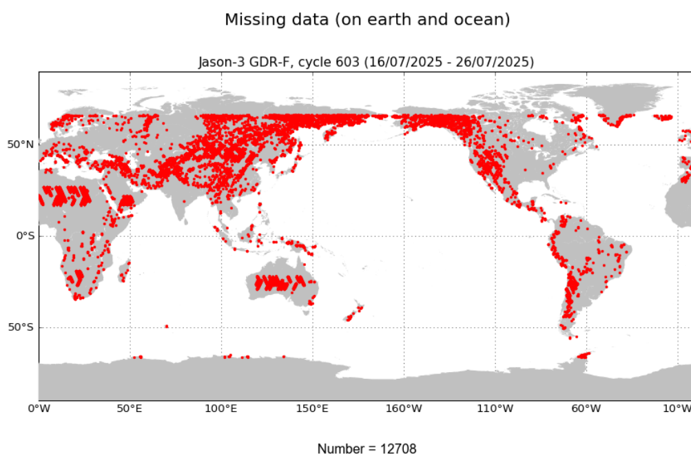
FIGURE 1 – Missing measurements for cycle 603.
