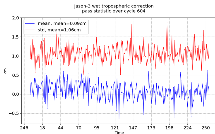
FIGURE 11 – Pass monitoring of wet troposphere differences between radiometer and ECMWF model for Jason-3 cycle 604
