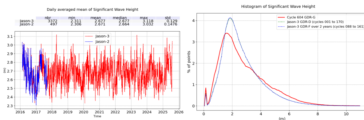
FIGURE 6 – Daily monitoring of Ku-band significant wave height for Jason-2 and Jason-3 (left) and histograms of Jason-3 (right).
