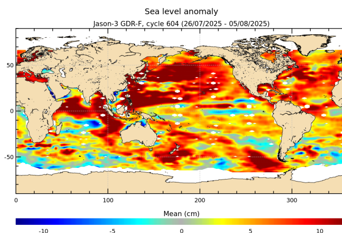
FIGURE 18 – Sea level anomaly relative to MSS for cycle 604.
