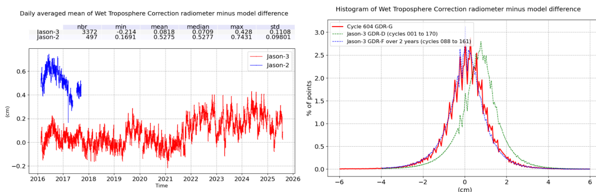
FIGURE 12 – Daily monitoring of wet troposphere differences between radiometer and ECMWF model for Jason-2 and Jason-3 (left) and histograms of Jason-3 (right).
