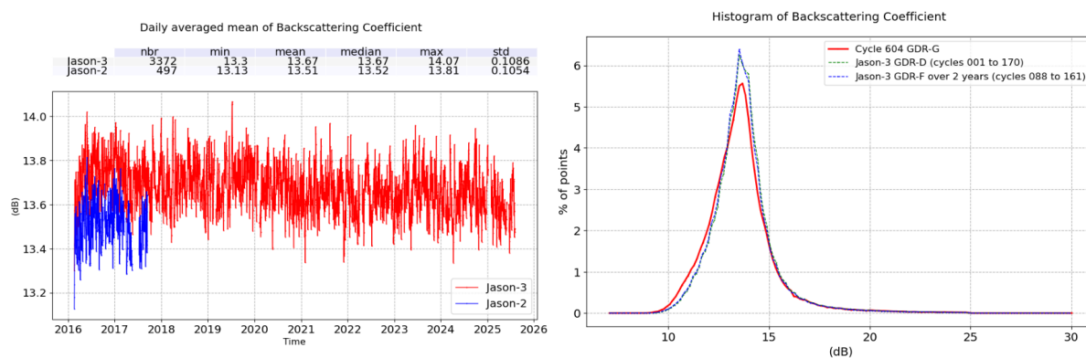
FIGURE 7 – Daily monitoring of Ku-band backscattering coefficient for Jason-2 and Jason-3 ( left ) and histograms of Jason-3 ( right ).
