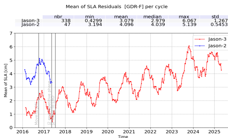
FIGURE 17 – Cyclic monitoring of mean SLA for Jason-3 and Jason-2.
