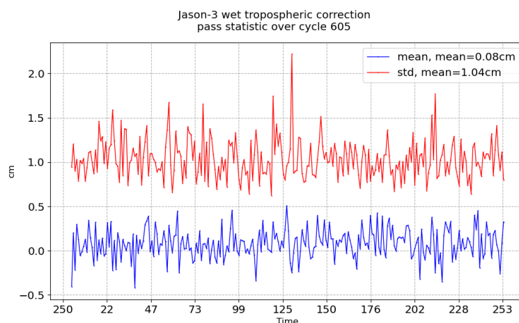
FIGURE 11 – Pass monitoring of wet troposphere differences between radiometer and ECMWF model for Jason-3 cycle 605
