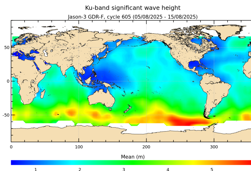
FIGURE 5 – Significant wave height for cycle 605.
