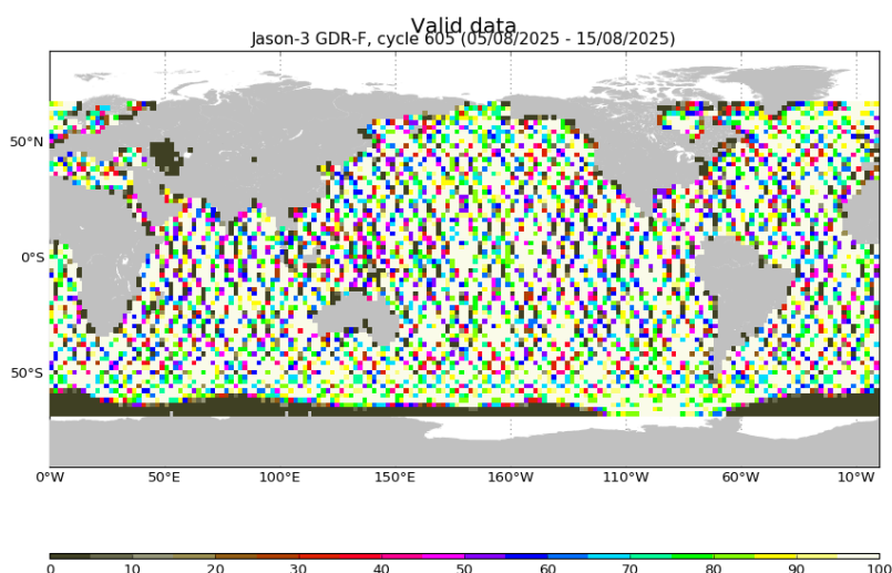
FIGURE 3 – Percentage of valid measurements for cycle 605.
