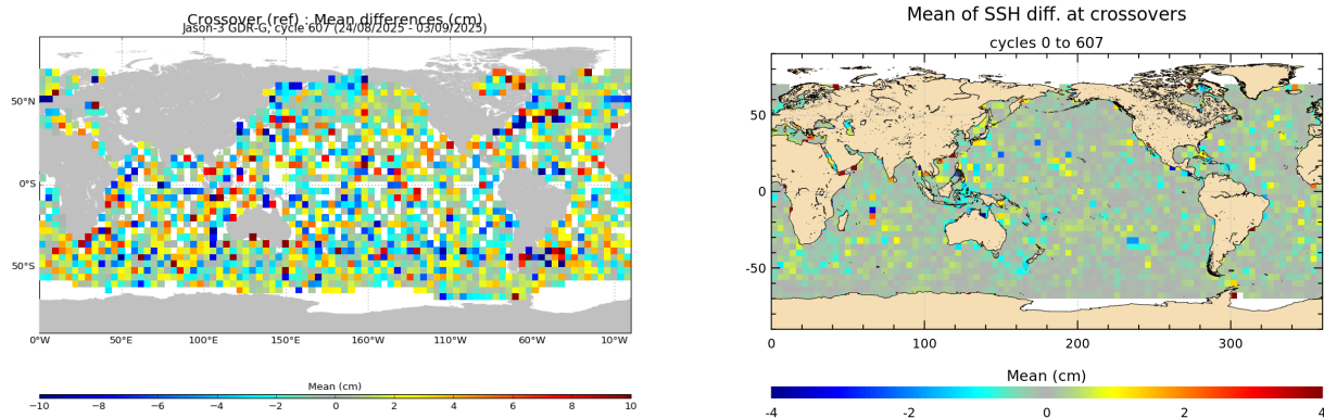
FIGURE 13 – Mean SSH at crossovers for cycle 607 (left) and over the whole Jason-3 period (right).
