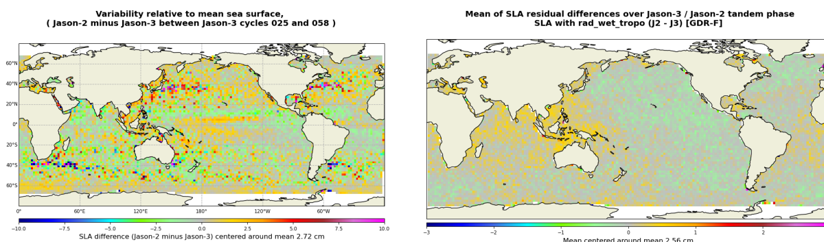
FIGURE 19 – Jason-2 – Jason-3 SLA differences averaged over Jason-3 period from cycle 025 until cycle 058 (left), and for tandem phase (cycle 001 to 023) (right).
