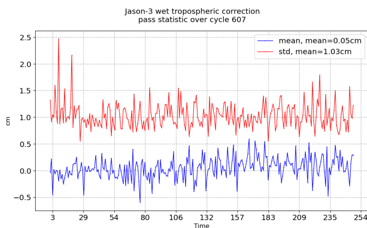
FIGURE 11 – Pass monitoring of wet troposphere differences between radiometer and ECMWF model for Jason-3 cycle 607
