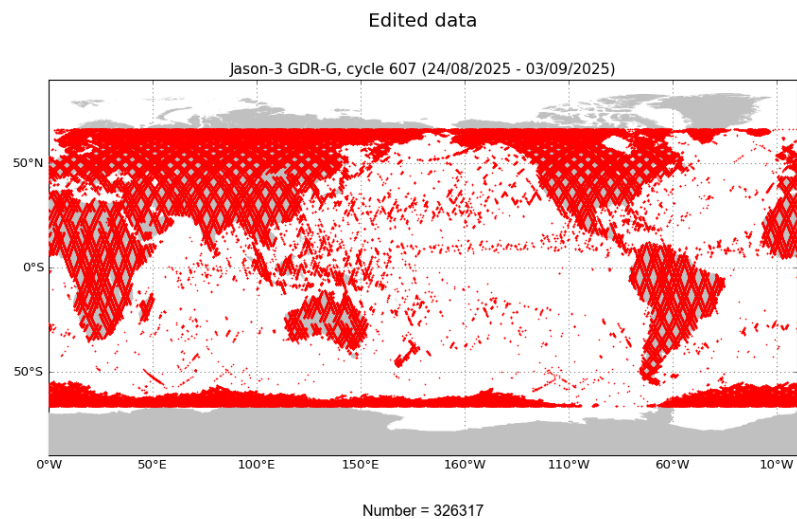
FIGURE 2 – Edited measurements for cycle 607.
