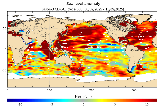
FIGURE 18 – Sea level anomaly relative to MSS for cycle 608.
