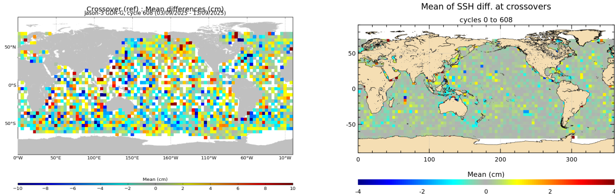
FIGURE 13 – Mean SSH at crossovers for cycle 608 (left) and over the whole Jason-3 period (right).
