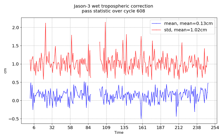
FIGURE 11 – Pass monitoring of wet troposphere differences between radiometer and ECMWF model for Jason-3 cycle 608
