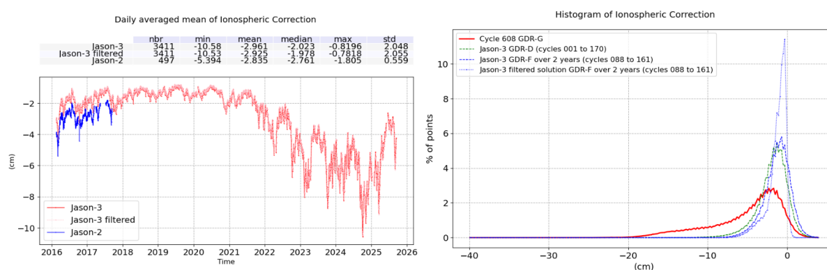
FIGURE 8 – Daily monitoring of dual-frequency ionosphere correction for Jason-2 and Jason-3 (left) and histograms of Jason-3 (right).
