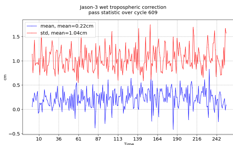
FIGURE 11 – Pass monitoring of wet troposphere differences between radiometer and ECMWF model for Jason-3 cycle 609
