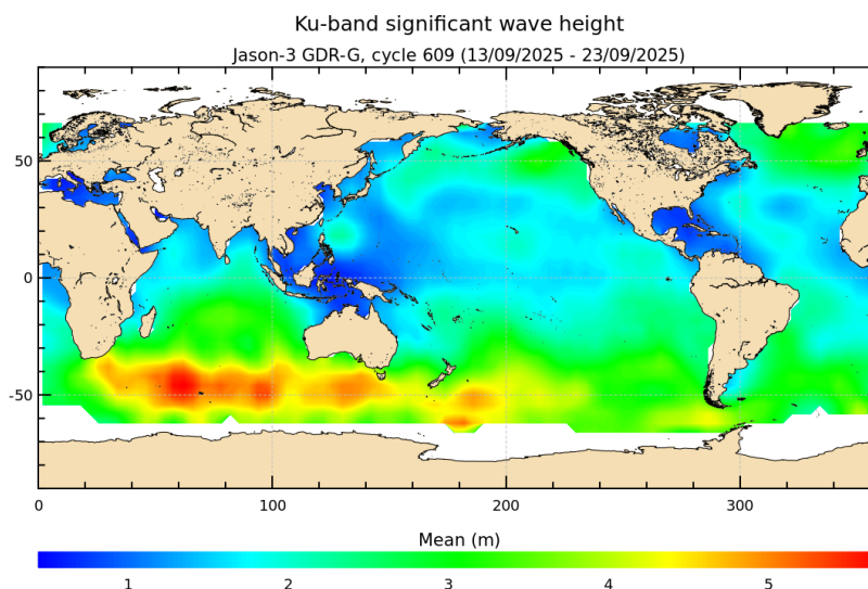
FIGURE 5 – Significant wave height for cycle 609.
