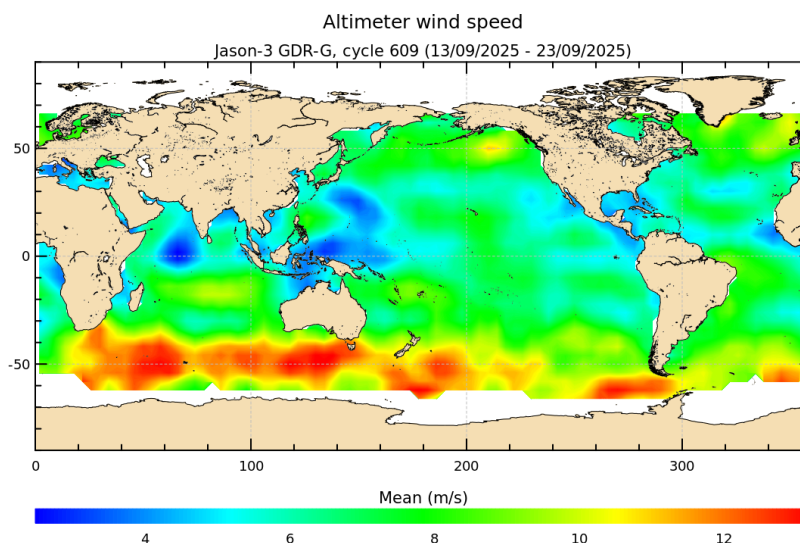
FIGURE 9 – Altimeter wind speed for cycle 609.
