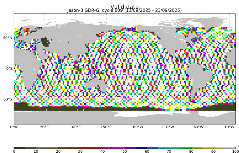
FIGURE 3 – Percentage of valid measurements for cycle 609.
