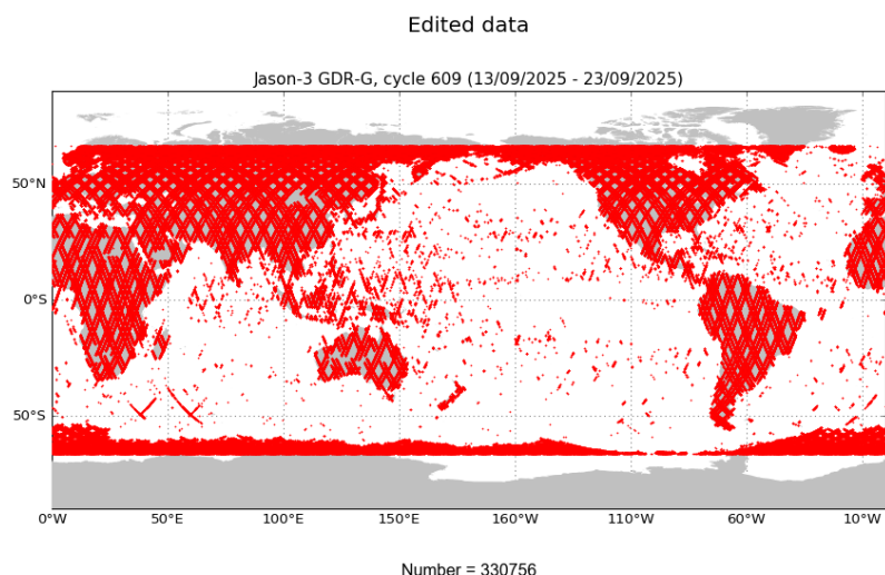
FIGURE 2 – Edited measurements for cycle 609.
