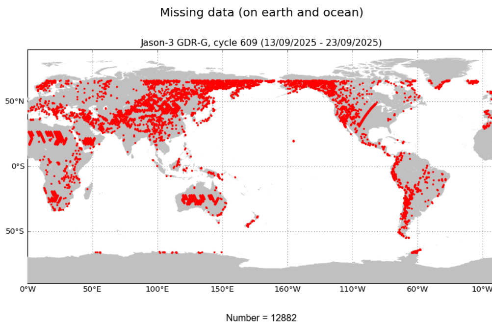
FIGURE 1 – Missing measurements for cycle 609.
