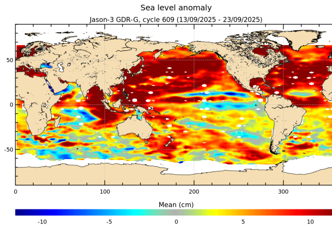
FIGURE 18 – Sea level anomaly relative to MSS for cycle 609.
