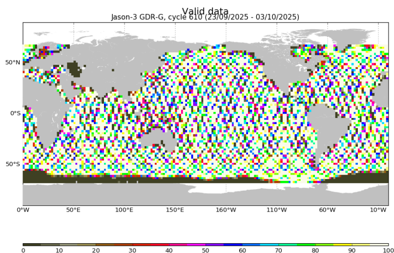
FIGURE 3 – Percentage of valid measurements for cycle 610.
