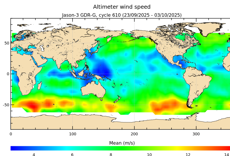
FIGURE 9 – Altimeter wind speed for cycle 610.
