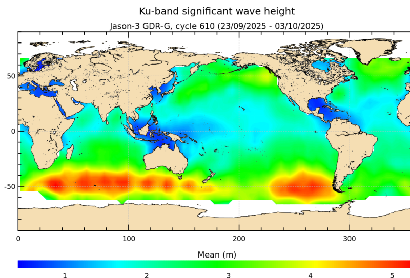
FIGURE 5 – Significant wave height for cycle 610.
