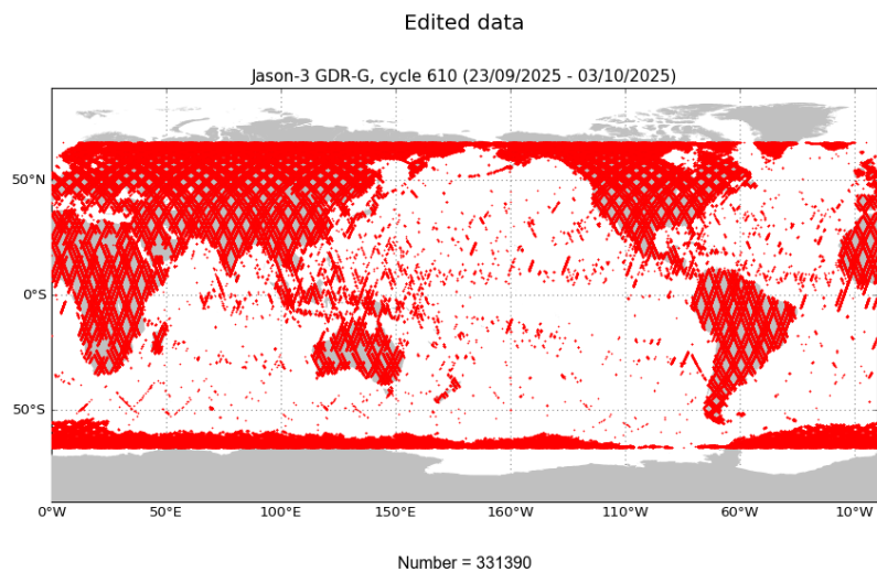
FIGURE 2 – Edited measurements for cycle 610.
