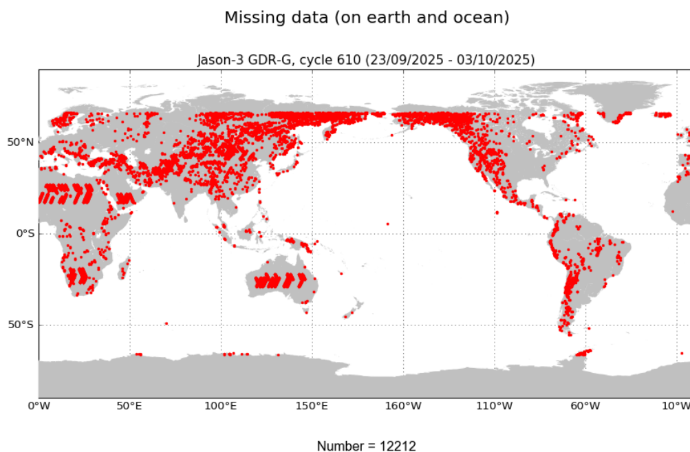
FIGURE 1 – Missing measurements for cycle 610.
