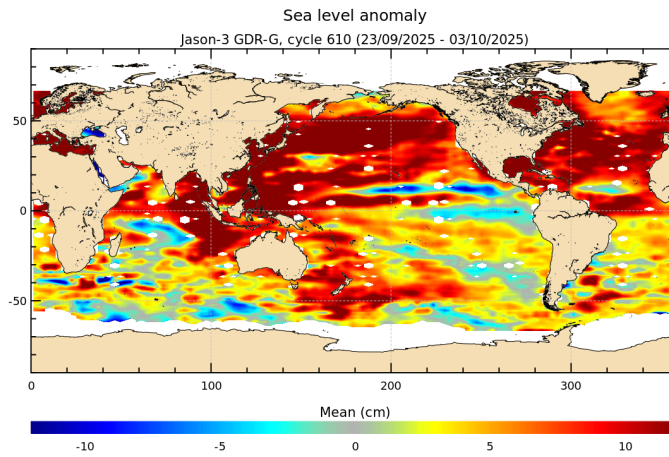
FIGURE 18 – Sea level anomaly relative to MSS for cycle 610.
