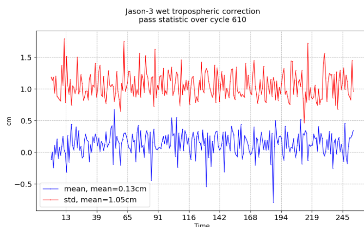
FIGURE 11 – Pass monitoring of wet troposphere differences between radiometer and ECMWF model for Jason-3 cycle 610
