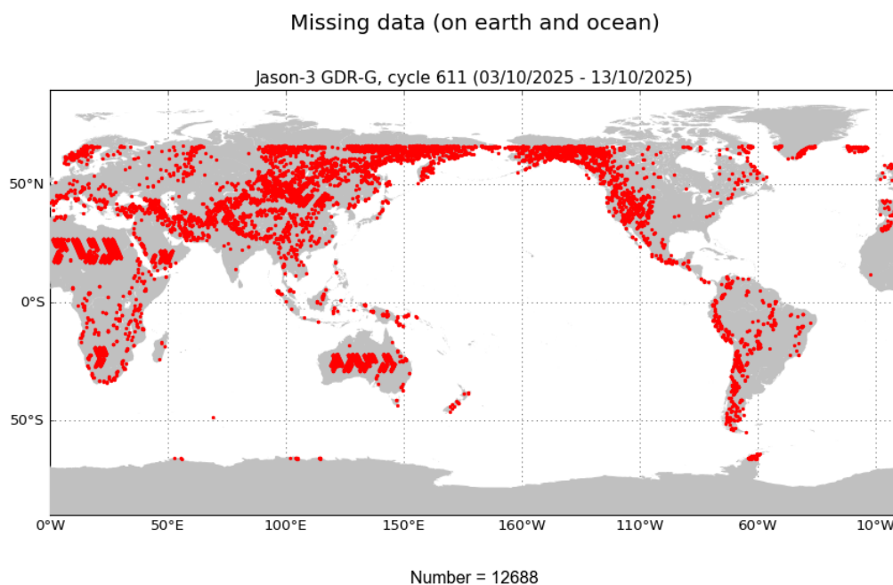
FIGURE 1 – Missing measurements for cycle 611.
