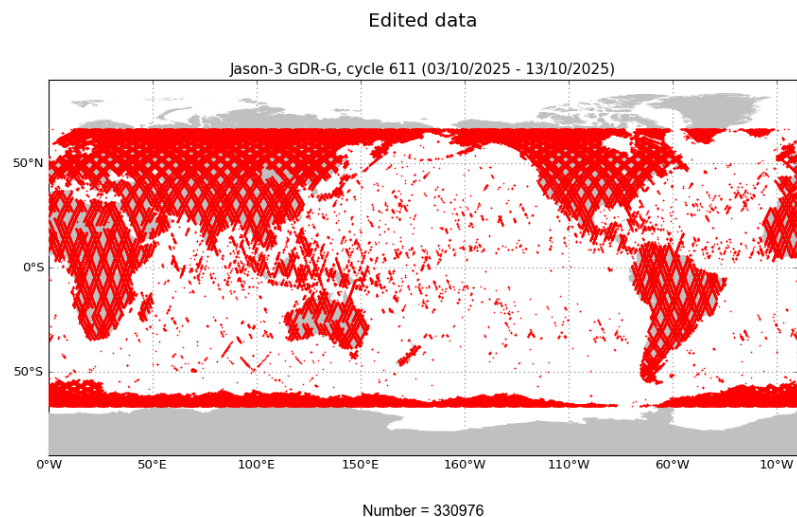
FIGURE 2 – Edited measurements for cycle 611.
