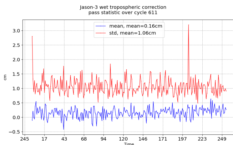
FIGURE 11 – Pass monitoring of wet troposphere differences between radiometer and ECMWF model for Jason-3 cycle 611
