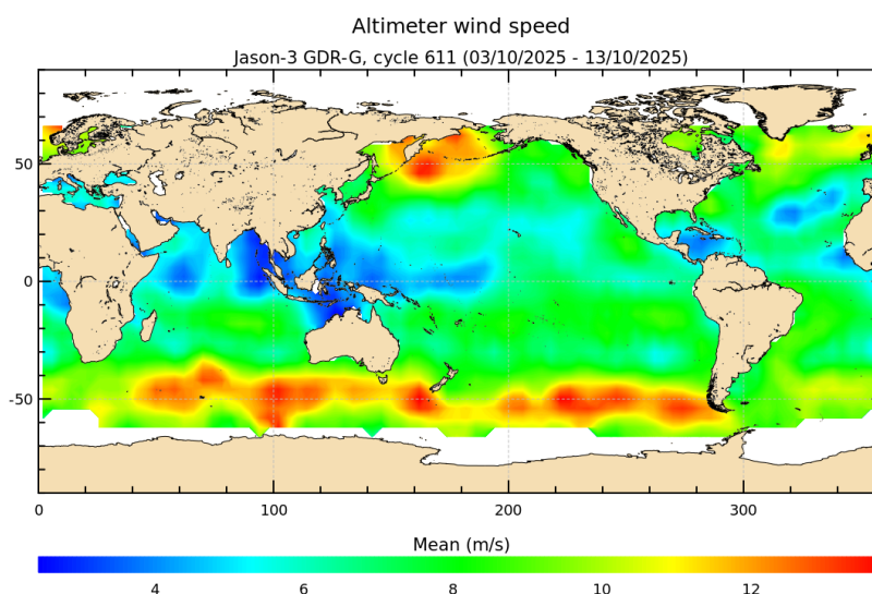
FIGURE 9 – Altimeter wind speed for cycle 611.
