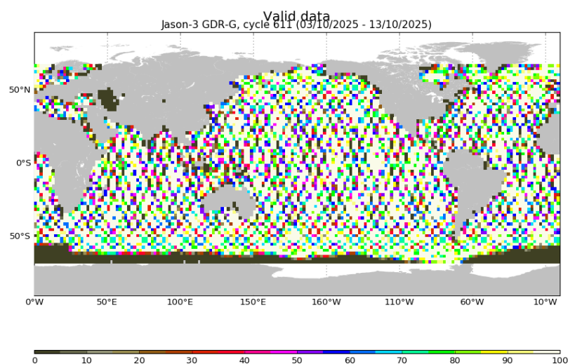
FIGURE 3 – Percentage of valid measurements for cycle 611.
