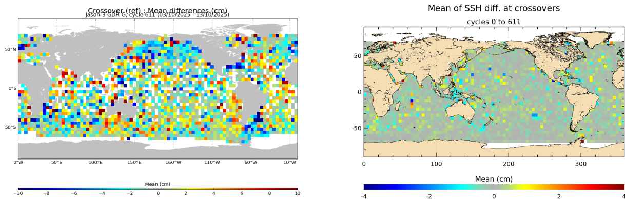
FIGURE 13 – Mean SSH at crossovers for cycle 611 (left) and over the whole Jason-3 period (right).
