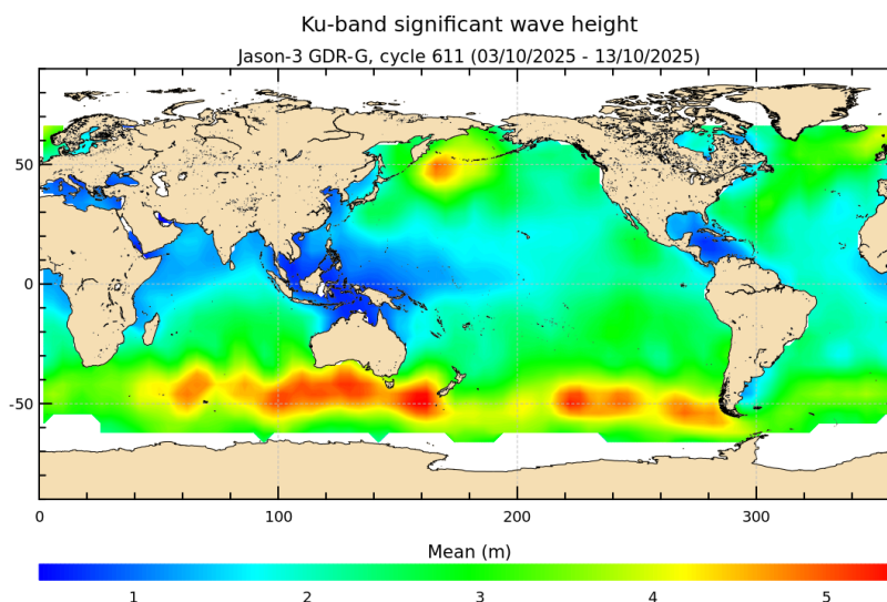
FIGURE 5 – Significant wave height for cycle 611.
