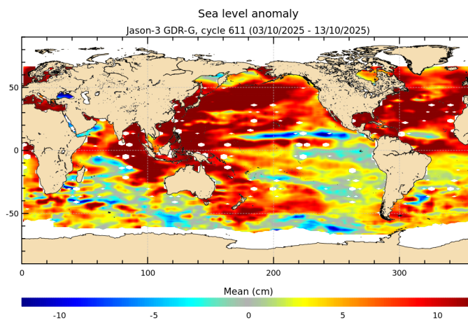
FIGURE 18 – Sea level anomaly relative to MSS for cycle 611.
