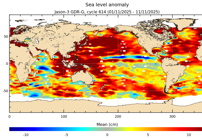
FIGURE 18 – Sea level anomaly relative to MSS for cycle 614.
