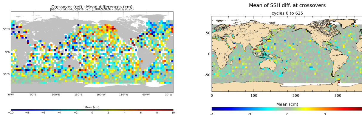
FIGURE 13 – Mean SSH at crossovers for cycle 625 (left) and over the whole Jason-3 period (right).
