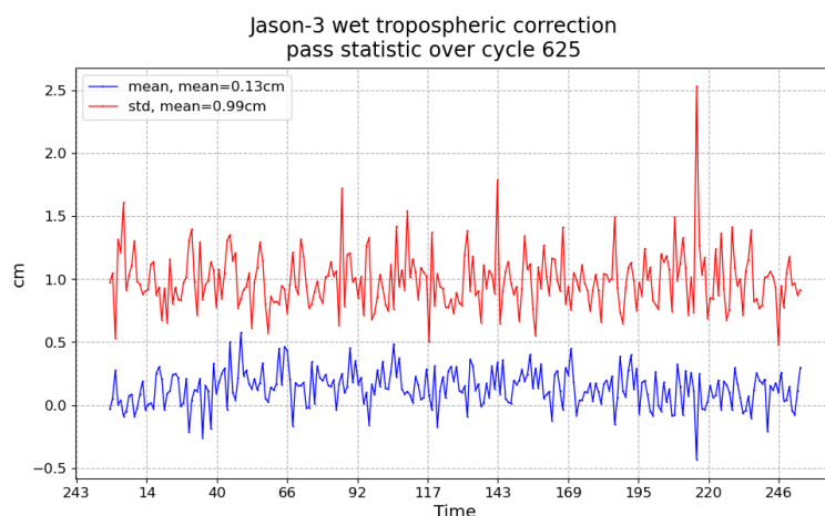
FIGURE 11 – Pass monitoring of wet troposphere differences between radiometer and ECMWF model for Jason-3 cycle 625
