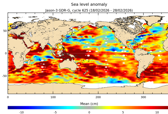
FIGURE 18 – Sea level anomaly relative to MSS for cycle 625.
