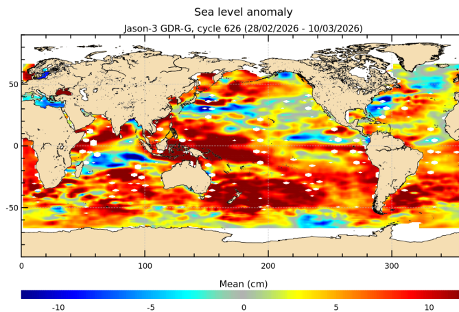
FIGURE 18 – Sea level anomaly relative to MSS for cycle 626.
