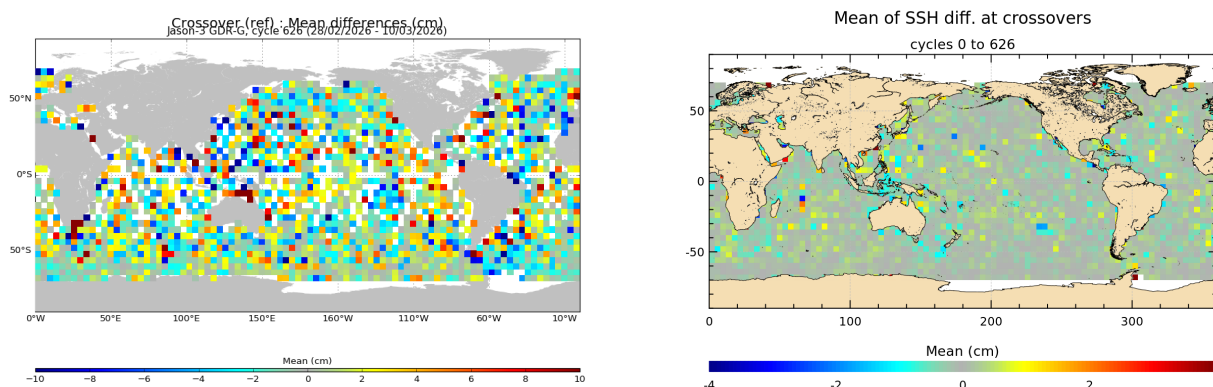
FIGURE 13 – Mean SSH at crossovers for cycle 626 (left) and over the whole Jason-3 period (right).
