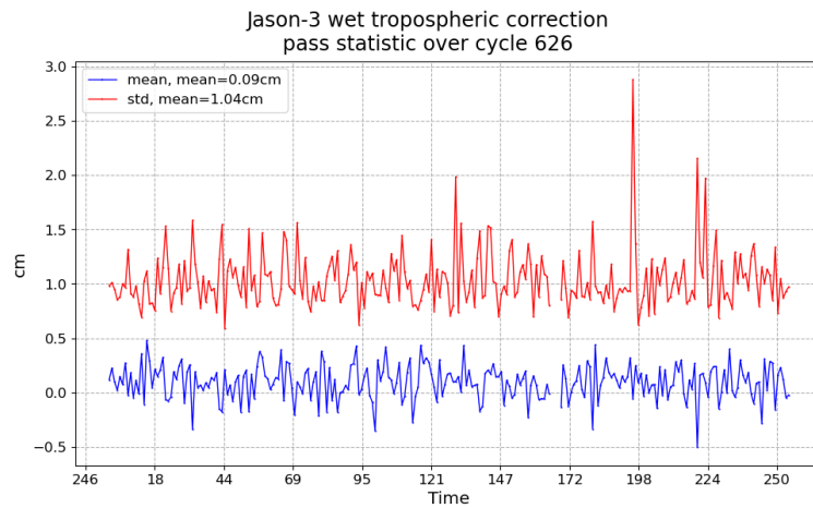
FIGURE 11 – Pass monitoring of wet troposphere differences between radiometer and ECMWF model for Jason-3 cycle 626
