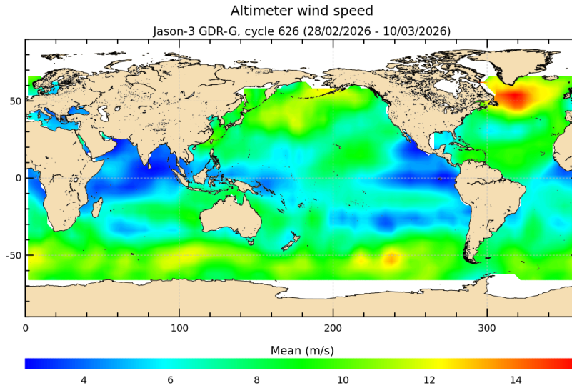
FIGURE 9 – Altimeter wind speed for cycle 626.
