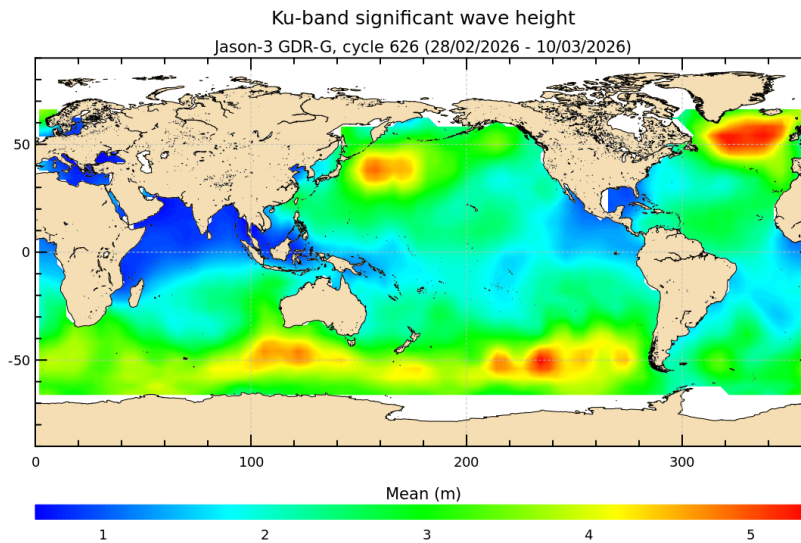
FIGURE 5 – Significant wave height for cycle 626.
